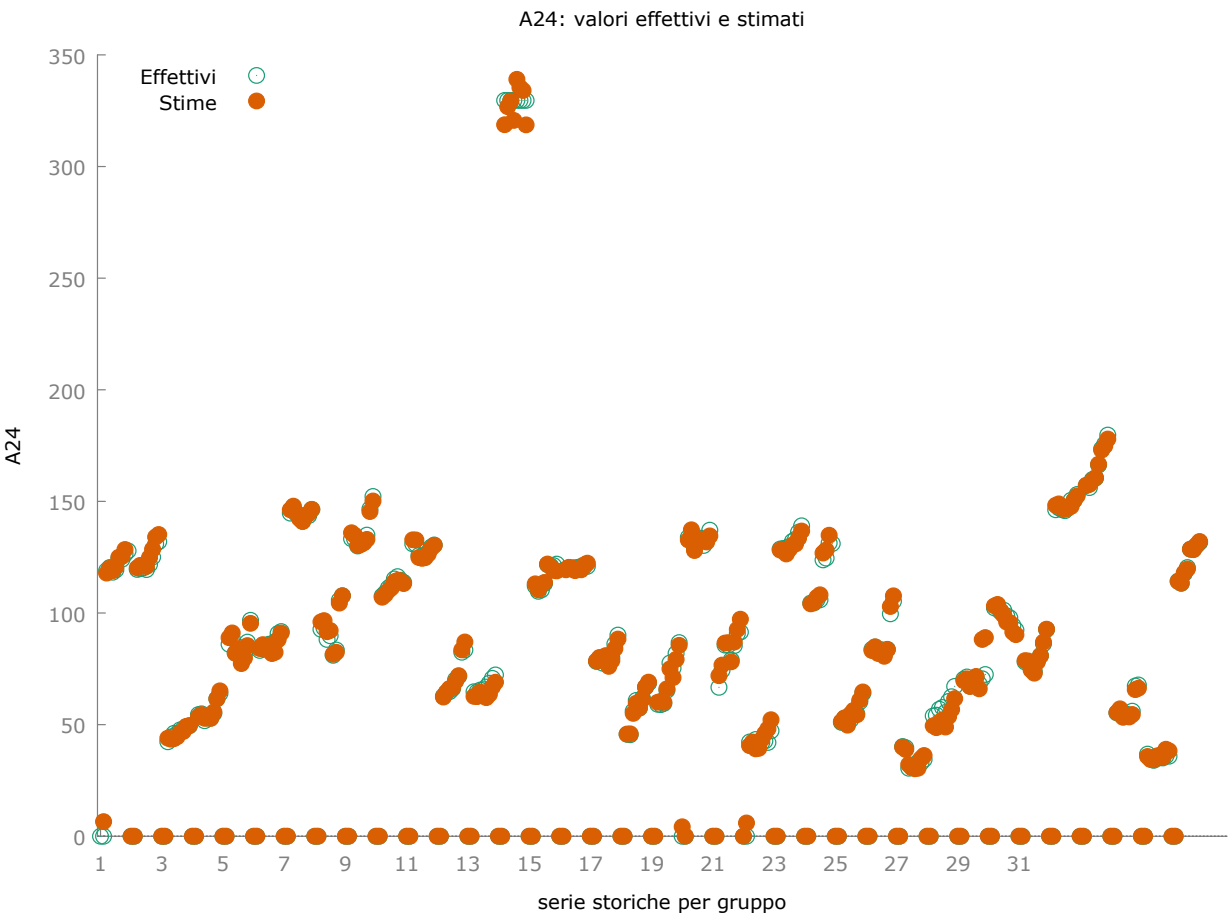
Clusterization
