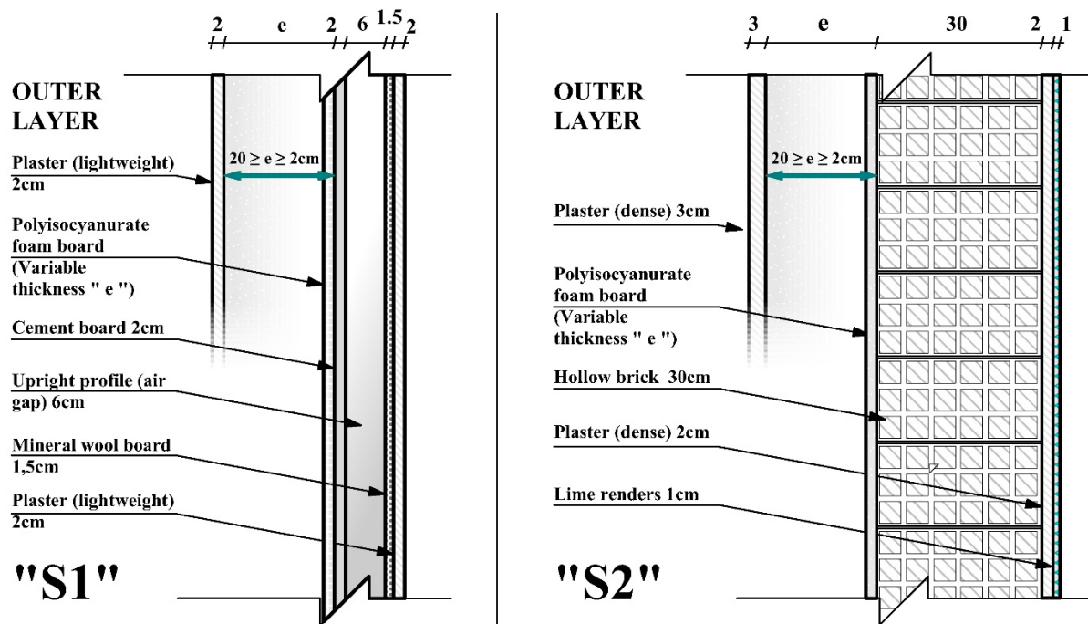
Figure 6. Building's external wall stratifications: scenario "S1": Low mass wall and scenario "S2": High mass wall.
