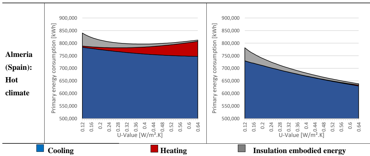
Figure 8. Building primary energy consumption in terms of heating and cooling for the 4 representative cities of the European context (Oslo, Bordeaux, Rome and Almeria)
