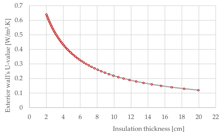
Figure 7. External wall's insulation thickness and related U-value
