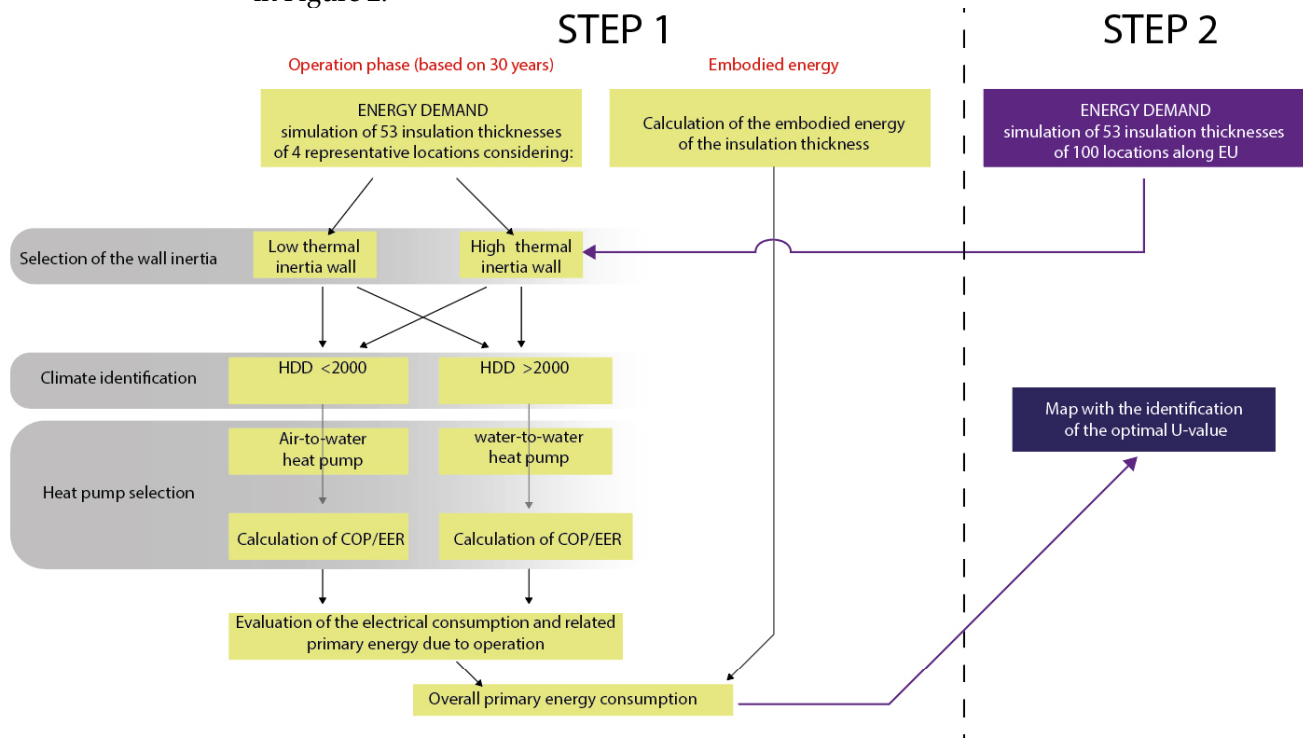
Figure 2. Research methodology workflow
