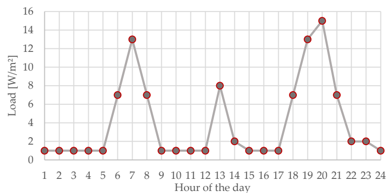
Figure 5. Internal gains daily profile
