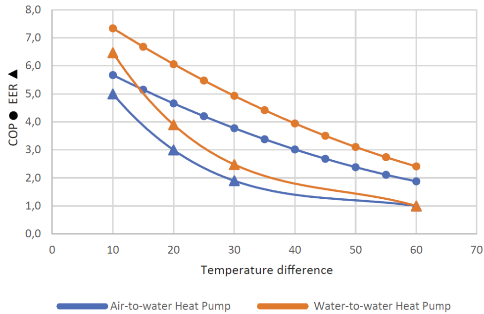
Figure 1. COP and EER reference trends as a function of temperature difference between sources
