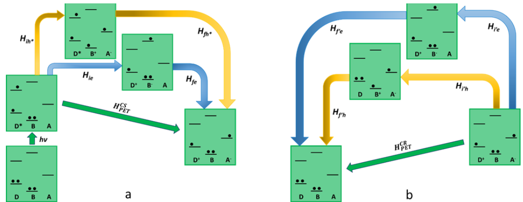
Figure 2: Schematic representation of oxidative photoinduced electron transfer in D-B-A dyads, according to superexchange. The states involved in the mechanism (virtual states pathways are described with blue and yellow arrows) are represented in terms of electronic configurations. On the left (photoinduced) charge separation is described while charge recombination is shown on the right.
