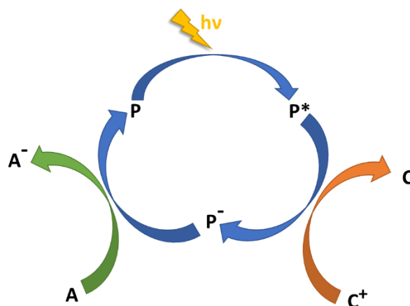
Figure 12: “Anti-biomimetic” scheme for catalyst oxidation performed by the Ru4/RuPOM system: reductive quenching of excited photosensitizer (P) by catalyst (C), followed by electron transfer to sacrificial acceptor (A) [69].
