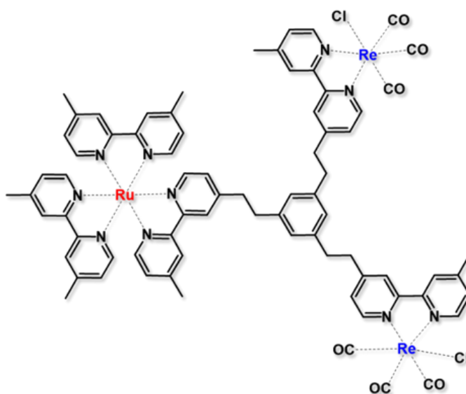
Figure 10: Structure of the supramolecular photocatalyst RuRe 2 for CO 2 reduction [61]
