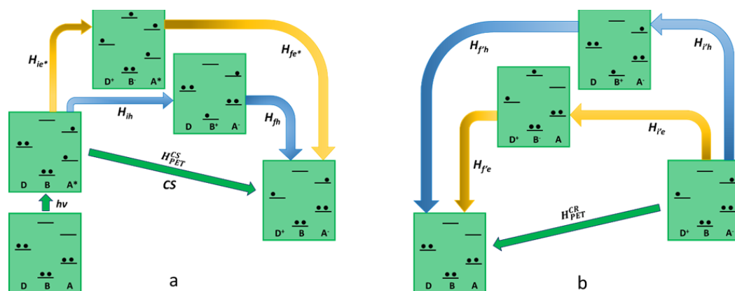
Figure 3: Schematic representation of reductive photoinduced electron transfer in D-B-A dyads, according to superexchange. The states involved in the mechanism (virtual states pathways are described with blue and yellow arrows) are represented in terms of electronic configurations. On the left charge separation is described while charge recombination is shown on the right.
