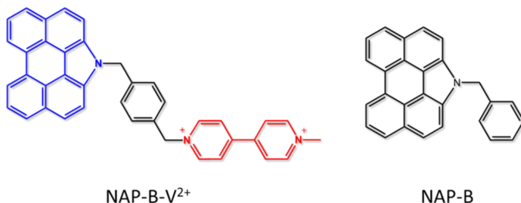
Figure 4: left ) D-B-A system constituted by a N-annulated perylene subunit (D), an aromatic central moiety used as a bridge (B) and a methylviologen derivative (A); right ) D-B model compound.
