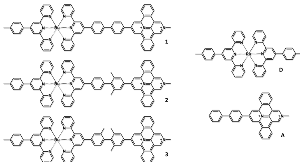
Figure 6: left) D-B-A structural formulas of the bichromophoric species systems; right) the model compounds concerning the donor (D) and acceptor (A) moieties.
