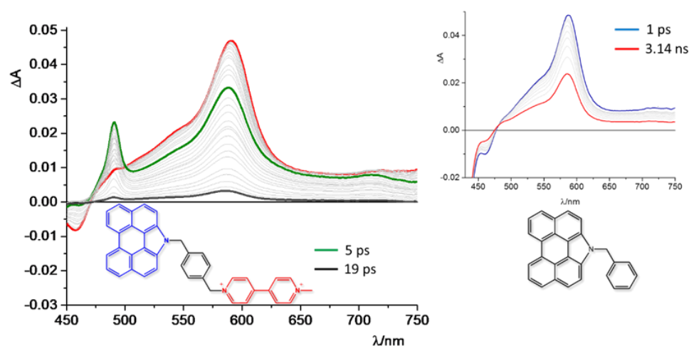
Figure 5: left) Transient absorption spectra of NAP-B-V 2+ dyad in acetonitrile; red spectrum was registered immediately after the pump, and time delays for the green and black spectra are given in the panel. right) Transient absorption spectra of NAP-B registered at different delays, indicated in panel.
