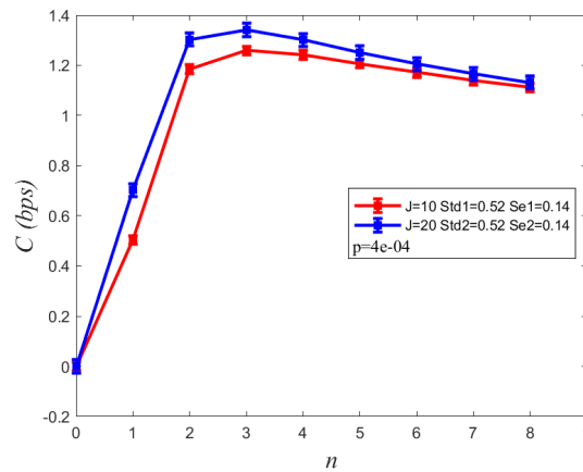
Figure 5. Comparison channel capacity C with the symbol duration T_b between two symbols, T_b = n * t_p , n=1, \dots, 8 . J denotes the photolysis reaction coefficient. Std and Se denote standard deviations and standard error, respectively.
