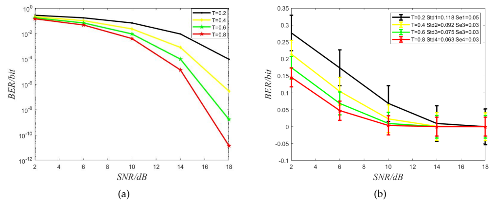
Figure 7. (a). Bit Error Ratio (BER) versus Signal Noise Ratio (SNR) with the different symbol interval. dB denotes the unit of SNR. (b). Std and Se denote standard deviations and standard error, respectively.
