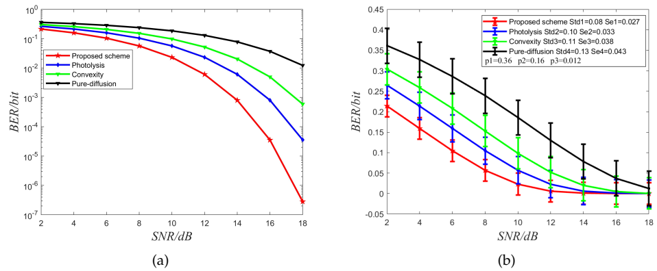
Figure 6. (a). Bit Error Ratio (BER) performance comparison of the proposed method with the methods in the previous reference. dB denotes the unit of Signal Noise Ratio (SNR). (b). Std and Se denote standard deviations and standard error, respectively. p_1 , p_2 and p_3 denote the p-values of the comparison between the proposed method with photolysis, convexity and pure diffusion, respectively.
