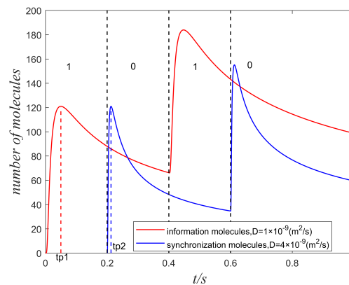
Figure 2. The information molecules and synchronisation molecules with different diffusion coefficients are transmitted along with symbol sequences 1010, where information molecules are released at the start of symbol "1", while the synchronisation molecules are released during the symbol "0". t/s denotes that the unit of time is seconds.
