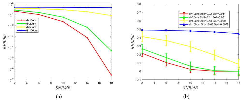
Figure 8. (a). Bit Error Ratio (BER) versus Signal Noise Ratio (SNR) with different distances. dB denotes the unit of SNR. (b). Std and Se denote standard deviations and standard error, respectively.
