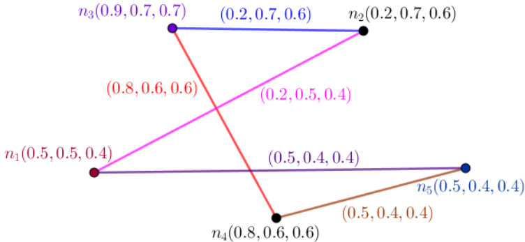
Figure 14. A Neutrosophic Graph in the Viewpoint of its Independent Number.
