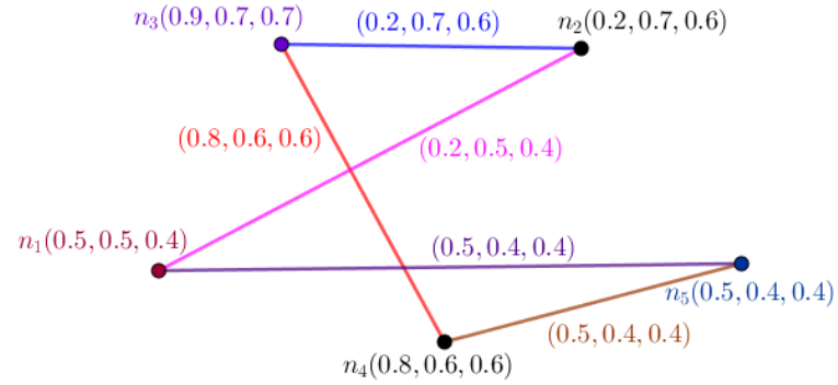
Figure 6. A Neutrosophic Graph in the Viewpoint of its Independent Number.
