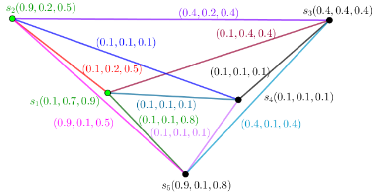
Figure 1. Black circles form a set which is 1-powerful alliance.
