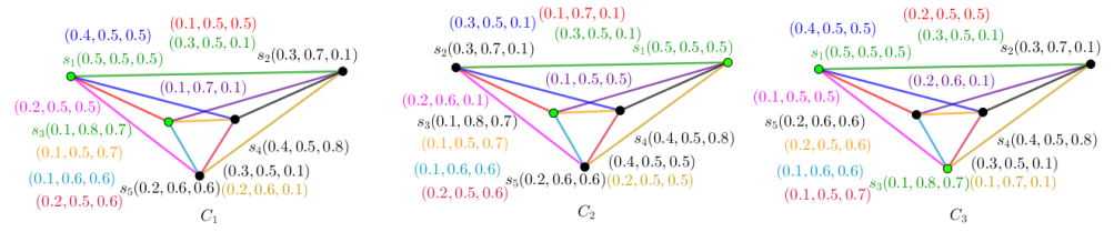
Figure 4. The set of black circles is minimal-global-offensive alliance.
