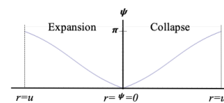
FIG. 13. Local light cone angles over time
