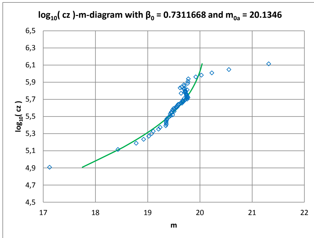
Figure 8. Magnitude-redshift diagram for 132,975 quasars according to M.-P. Véron-Cetty et al. [2].
