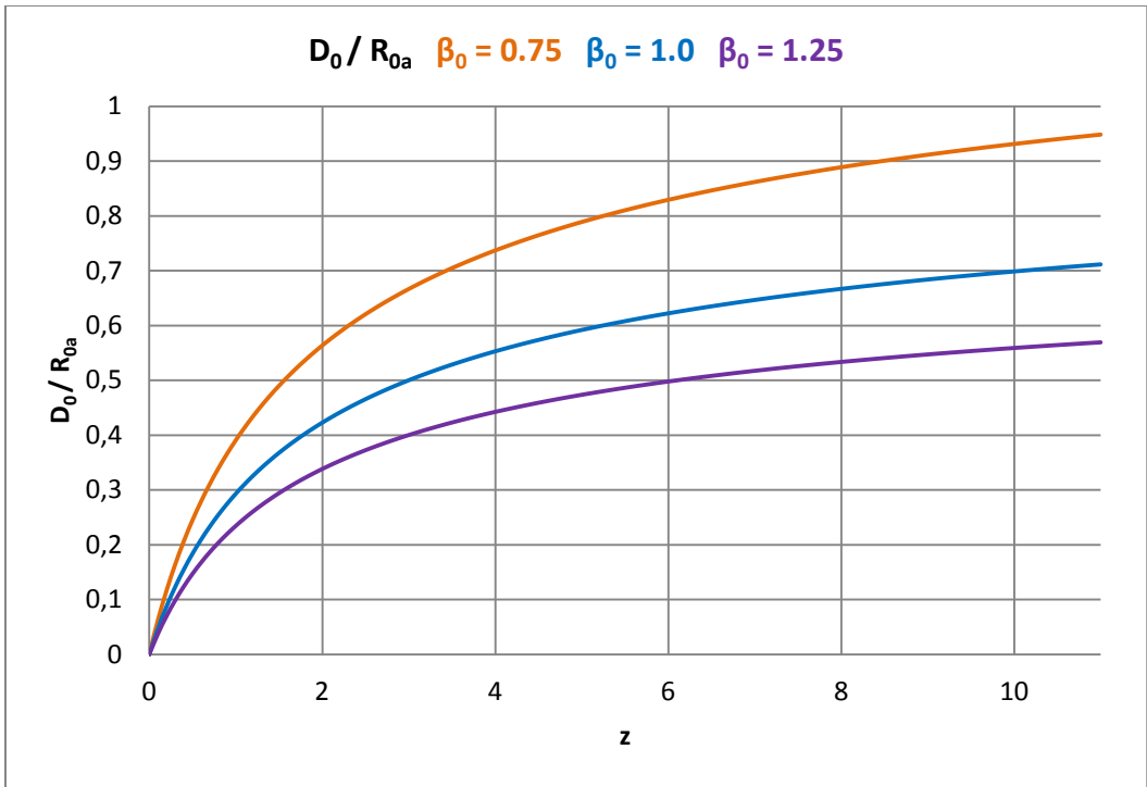
Figure 4. Today's ( t_0 ) redshift distance D_0 normalized to the distance R_{0a} for various values of the parameter \beta_0 .
