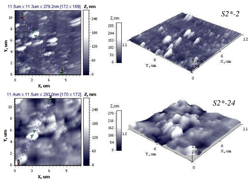
Figure 8. AFM images of cadmium chalcogenide layers on PA 6.
