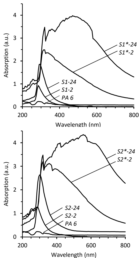
Figure 3. UV-Vis absorption spectra of PA 6, chalcogenized samples in the solutions of \text{H}_2\text{TeS}_4\text{O}_6 and samples with the layers of cadmium chalcogenides.
