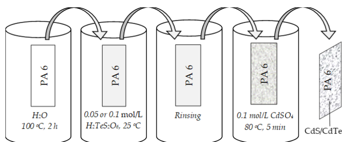
Figure 1. Schematics of cadmium chalcogenide layers formation procedure.
