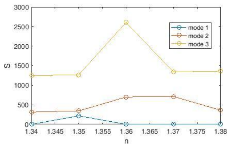
Fig.15. Plasmonic sensor sensitivity coefficient diagram in water
