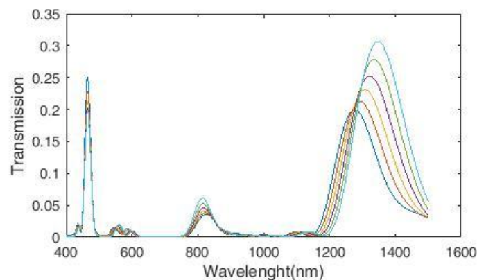
Fig.9. Transmission spectra of a plasmonic refractive index sensor
