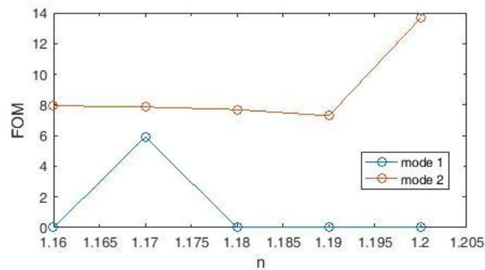
Fig.6. Plasmonic sensor FOM diagram
