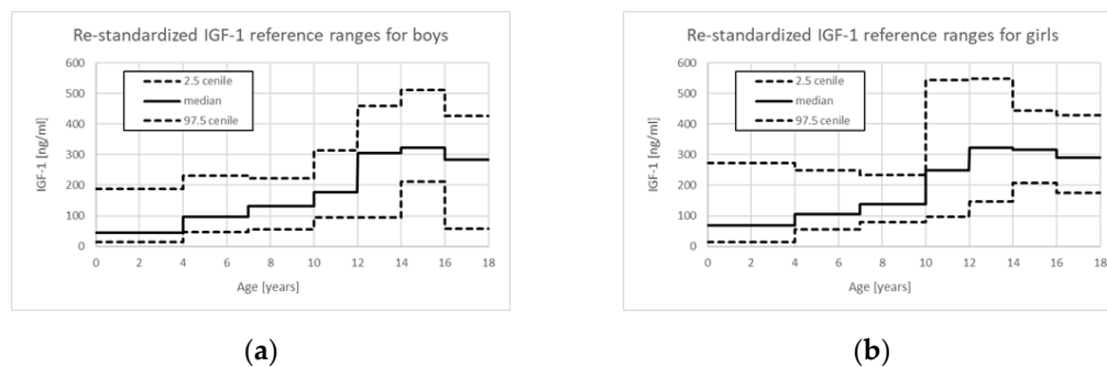
Figure 1. Centile charts based on Pediatric reference ranges for re-standardized IGF-1 assays provided for IMMULITE 2000 Immunoassay System [59]. (a) for boys; (b) for girls.
