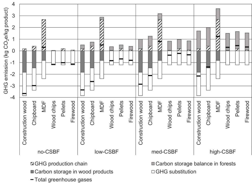
Figure 2. Greenhouse gas balances of wood products in different carbon storage balance scenarios in forests. MDF = medium-density fiberboard, CSBF = carbon storage balance in forests. See explanation of the scenarios no-CSBF, low-CSBF, med-CSBF and high-CSBF in Table 3.
