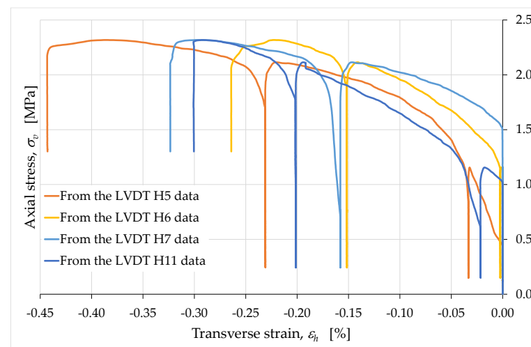
Figure 14. Axial stress/transverse strain curves acquired by the horizontal LVDTs between the ribs.
