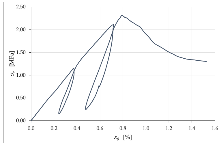
Figure 20. Curve of the axial stress, \sigma_v , with respect to \varepsilon_\theta (apparent volumetric strain).
