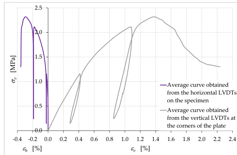
Figure 18. Average curves of axial stress with respect to axial and transverse strain.
