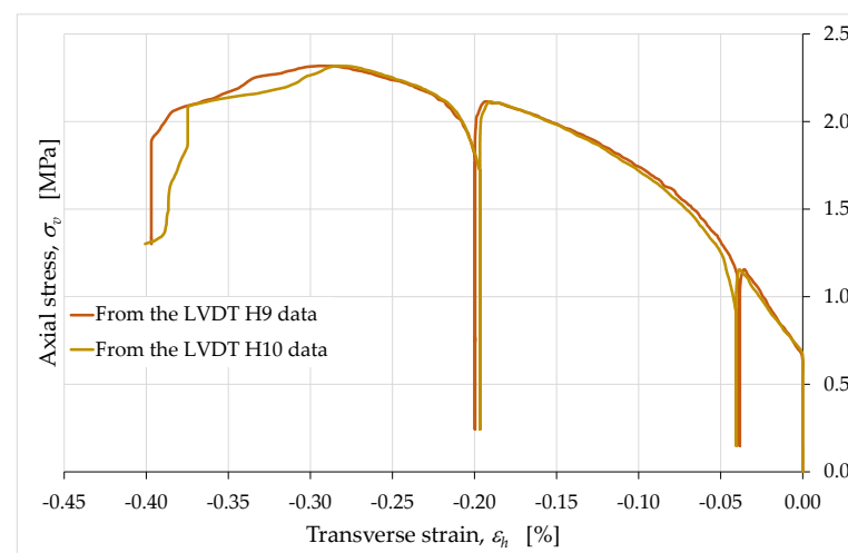
Figure 15. Axial stress/transverse strain curves acquired over the entire length of the long side faces.
