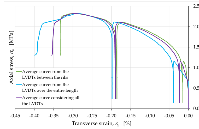
Figure 16. Average curves of axial stress with respect to transverse strain, obtained from the relative displacements over the inter-rib length and over the entire length of the long side faces.
