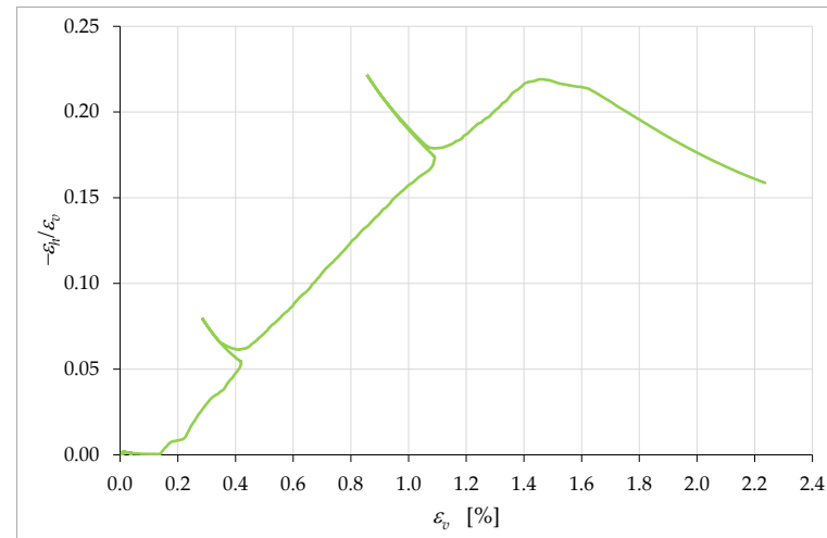
Figure 19. Curve of \nu (apparent Poisson's modulus) with respect to the axial strain, \varepsilon_v .
