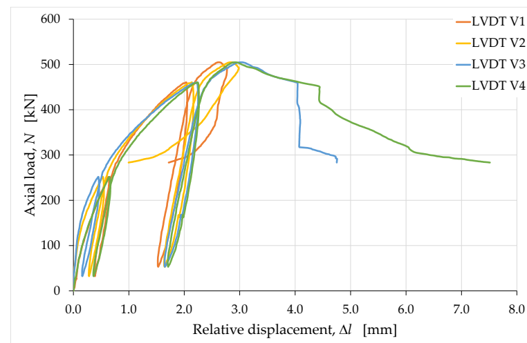
Figure 8. Load/displacement curves acquired along the vertical edges of the specimen.
