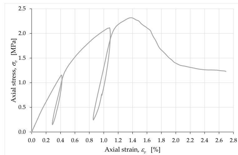
Figure 25. Complete average curve of the axial stress with respect to the axial strain, obtained from the acquisitions of the LVDTs placed between the corners of the metal plates for the distribution of the load.
