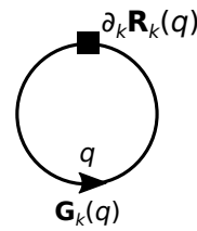
Figure 1. Diagrammatic representation of the Wetterich equation (19). The solid line represents the propagator \mathbf{G}_k = (\mathbf{\Gamma}_k^{(2)} + \mathbf{R}_k)^{-1} and the square represents the insertion \partial_k \mathbf{R}_k .
