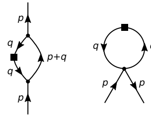
Figure 3. Diagrams that contribute to the flow of the 2-point function \Gamma_k^{(2)} . The internal lines correspond to propagators \mathbf{G}_k , while the black squares correspond to the insertion \partial_k \mathbf{R}_k .
