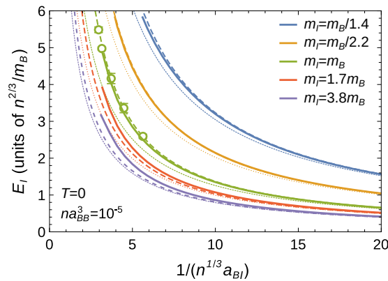
Figure 8. Polaron energy E_I at zero temperature as a function of (n^{1/3}a_{BI})^{-1} for na_{BB}^3 = 10^{-5} , where n is the density of the bath. The different colours correspond to energies of impurities with different masses. The thin dotted lines correspond to the MF solutions (61), the thin dashed lines include the first perturbative correction (61), the solid lines correspond to FRG calculations, and the circles correspond to MC simulations for m_I = m_B from Ref. [45].
