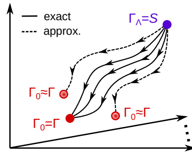
Figure 2. Illustration of the RG flow of \Gamma_k in parameter space [63]. The solid curves represent exact flows with different regulator choices. The dashed curves represent flows with a truncated ansatz.
