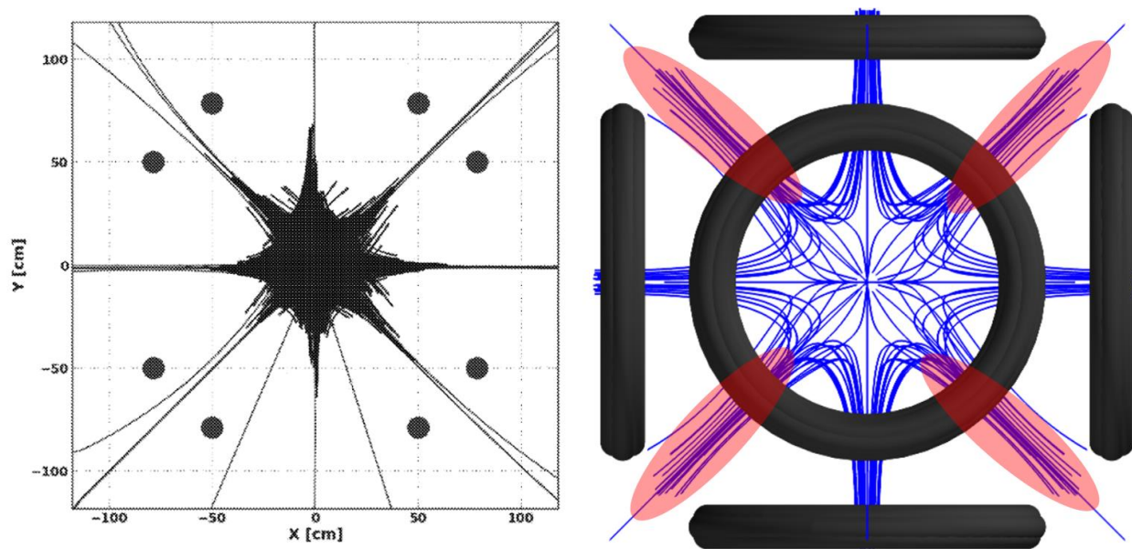
Figure 3. (left) shows numerically computed electron trajectories for the six coil cusp magnetic configuration from Dr. Park's patent application; (right) cross-section side view the of polyhedral coil mirroring what is depicted in the left image to present where electron loss occurs.
