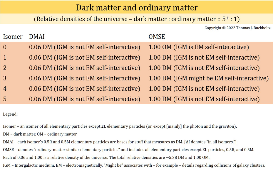
Figure 5: Dark matter density of the universe and ordinary matter density of the universe. The DM (or, dark matter) relative densities sum to approximately 5.38 times the OM (or, ordinary matter) relative density. Across isomers, the masses of similar elementary particles are identical. However, for charged leptons, associations between flavour and mass are not necessarily identical. Differences in associations between charged-lepton flavours and charged-lepton masses lead to differences - between isomers - in the evolution of stuff that associates with respective isomers. The stuff that associates with at least four DM isomers of elementary particles evolves so that the associated IGM (or, intergalactic medium) does not interact electromagnetically much with itself, compared to the interactivity of OM IGM. The lack - across at least four DM isomers - of much IGM electromagnetic self-interaction might associate with observations regarding the Bullet Cluster collision of two galaxy clusters.
