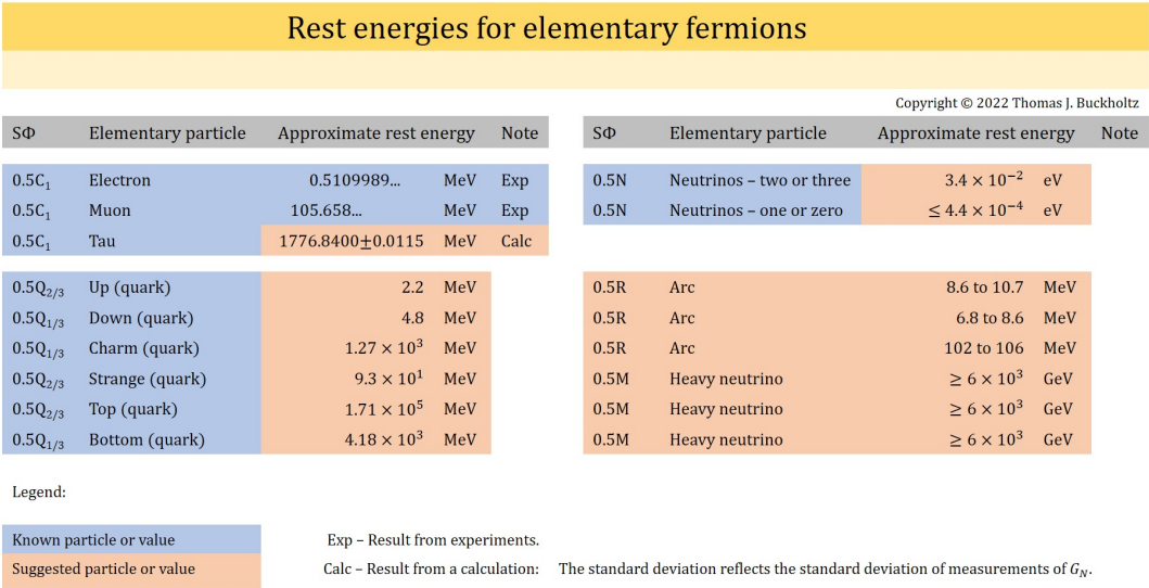
Figure 10: Possible rest energies for elementary fermions. Eight standard deviations of the calculated tau rest energy fit within one standard deviation of the measured tau rest energy. The calculated quark rest energies comport with experimental results. Results regarding neutrinos comport with the notion of three (not heavy) neutrinos and with astrophysics data. Our work suggests possible ranges for the rest energies of each of the three possible arc (or, 0.5R) elementary fermions. Our work suggests two possible lower limits for the rest energies of the three possible heavy neutrino elementary fermions. The figure shows one of those possible lower limits. The other possible lower limit is \sim 2.5 \times 10^9 GeV.
