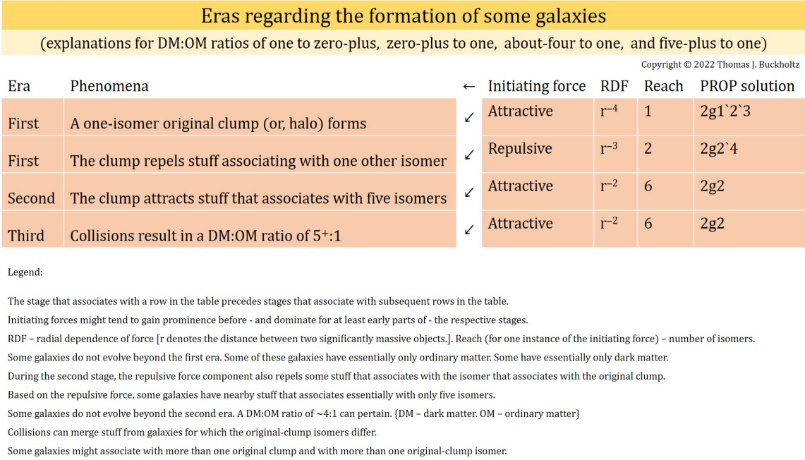
Figure 8: Suggested eras and suggested DM:OM ratios for galaxies. The stage that associates with a row in the figure precedes stages that associate with subsequent rows in the figure. For each row, the leftmost two columns associate with aspects of the stage. The rightmost four columns associate with a noteworthy cause for the stage. The noteworthy cause might gain prominence before the stage starts. Some galaxies do not transit beyond some stages. Our work points to possible propensities for nature to form galaxies with DM:OM ratios of approximately one to zero-plus (that is, dark matter galaxies), five-plus to one, four to one, and zero-plus to one. Galaxies that both had more than one original clump and had three original-clump isomers might tend to cease star formation earlier than do some other galaxies.
