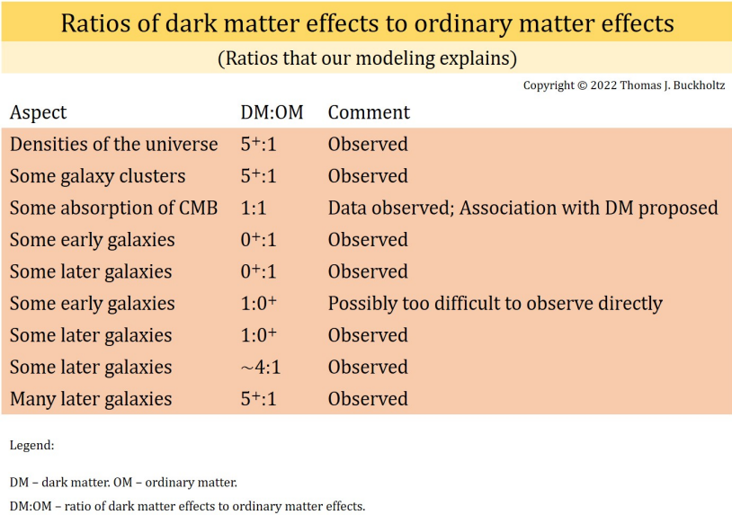
Figure 3: Ratios of dark matter effects to ordinary matter effects. For each ratio except two of the ratios, the following three sentences pertain. People have observed the ratio. People attribute the so-called dark matter effects to dark matter. Our modeling explains the ratio. Regarding some specific depletion of cosmic microwave background radiation (or, CMB), people have observed the ratio, some people speculate that the effects that people might not attribute to ordinary matter are effects of dark matter, and our modeling suggests that non-ordinary-matter effects are effects of dark matter. We use the two-word term early galaxies to include galaxies observed at redshifts of at least (and possibly somewhat less than) seven. Most relevant data about later galaxies pertains to galaxies observed at redshifts considerably less than seven. The three-word term dark matter galaxy pertains to a galaxy for which the DM:OM ratio (or, ratio of dark matter effects to ordinary matter effects) is one to zero-plus. Possibly, current techniques are not adequately sensitive to detect early dark matter galaxies.
