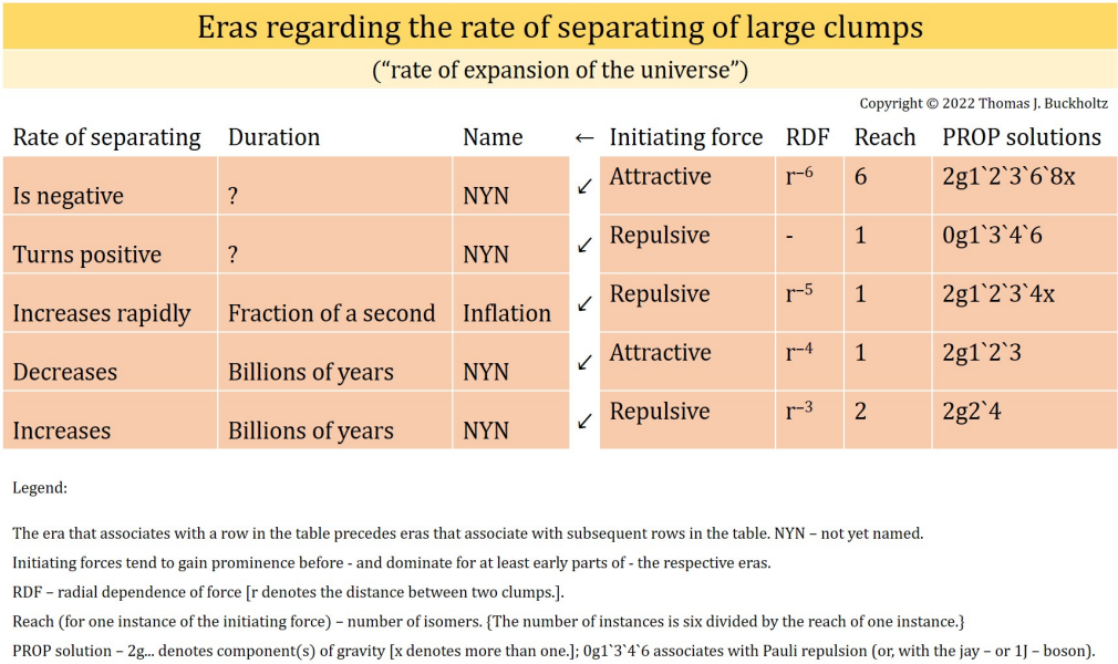
Figure 7: Suggested and known eras regarding the rate of expansion of the universe. The era that associates with a row in the figure precedes eras that associate with subsequent rows in the figure. For each row, the leftmost three columns describe aspects of the era. The rightmost four columns associate with a noteworthy cause for the era. Generally, the noteworthy cause gains prominence before the era starts. Our work proposes the first two eras to which the image alludes. Other work and our work suggest the era of inflation. Other work and our work model aspects of the two multi-billion-years eras. Our work might explain seeming difficulties that other work seems to exhibit regarding modeling aspects of the current multi-billion-years era of increasing rate of separation.
