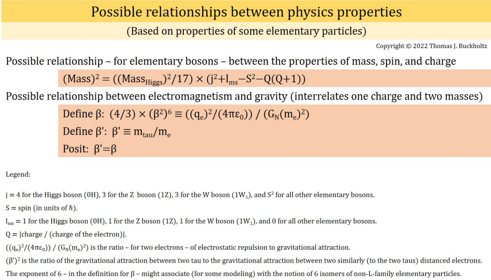
Figure 9: Possible relationships between physics properties. The boson-centric relationship might pertain for all known elementary bosons and for all new elementary bosons that we suggest. The possible relationship between electromagnetism and gravity enables computing a tau mass that is compatible with experimental results.
