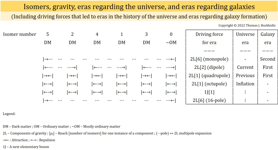
Figure 6: Isomers of elementary particles, components of gravity, eras in the evolution of the universe, and eras in the evolution of galaxies. Some current galaxies did not transit beyond the first era regarding the evolution of galaxies.
