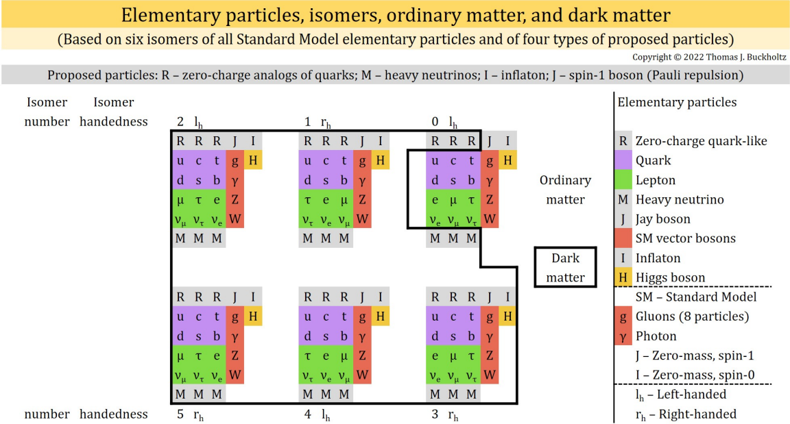
Figure 4: Elementary particles, isomers, ordinary matter, and dark matter. For counterpart elementary particles (across the six isomers), the masses are the same. Here, the word counterpart refers to positions in the six similar arrays of symbols for elementary particles. For counterpart elementary particles, the magnitudes of the charges are the same. For counterpart leptons, the flavours are not necessarily the same. For each known elementary particle, this figure uses popular symbols. Here, the lower-case letter g associates with gluons. Here, the symbol \gamma associates with the photon. The figure de-emphasizes the would-be graviton (or, 2L particle), the might-be 3L particle, and the might-be 4L particle. The figure de-emphasizes components - of the photon (or, 1L particle) for which the reaches exceed one.
