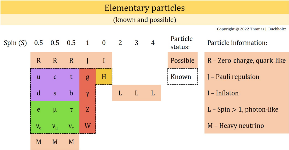
Figure 2: Known and suggested elementary particles. The figure uses popular symbols for the known elementary particles. The following sentences discuss symbols for and notions about suggested new elementary particles. (The number S in a symbol S\Phi , associates with elementary-particle spin in units of \hbar .) 0.5R associates with three spin-one-half zero-charge analogs to quarks. 1J associates with a spin-one zero-charge boson that associates with Pauli repulsion. 0I associates with a spin-zero inflaton. 2L associates with a possible spin-two graviton. 3L associates with a possible spin-three relative of the photon and the graviton. 4L associates with a possible spin-four relative of the photon and the graviton. 0.5M associates with three spin-one-half heavy neutrinos.
