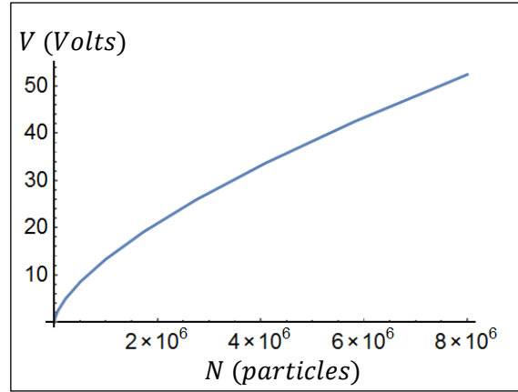
Fig.4: Electric potential produced by positive particles in fixed SCL arrangement, with equal spacing ( 2.66 \times 10^{-6} m ) as evaluated in Equation (10).
