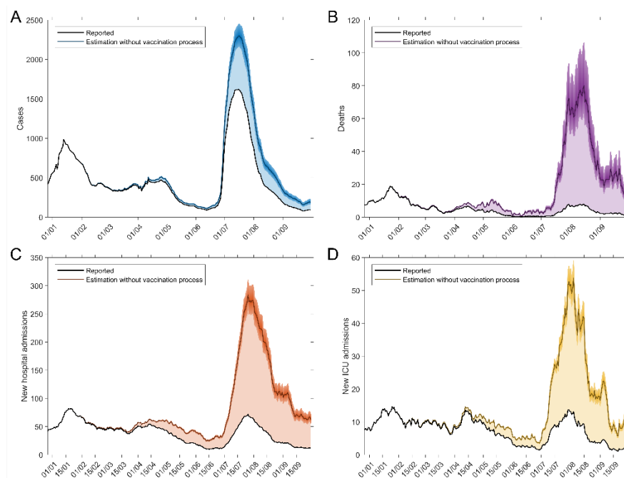
Figure 2. Epidemiological developments with and without the effect of vaccines. (A) Cases. (B) Deaths. (C) New hospitalizations. (D) New ICUs. Base case.
