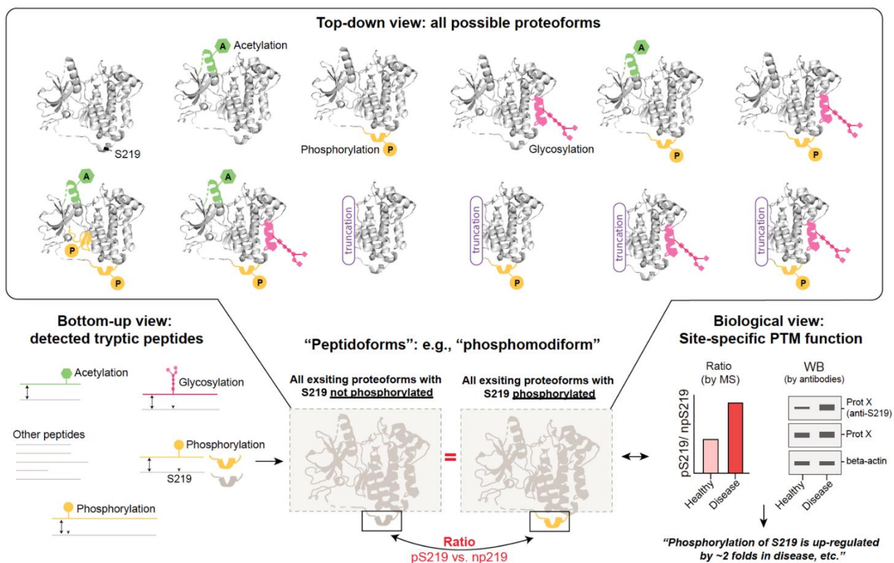
Figure 1. The top-down and bottom-up views for studying PTM biology. A virtual example of protein X (representing any protein) is shown. This protein X can be modified by different enzymes at different amino acid residues, forming a variety of possible proteoforms carrying acetylated, phosphorylated, or glycosylated sites and even the combinatorial PTMs in the cells. Additionally, the mRNA alternative splicing could create some truncated proteoforms of X. In bottom-up proteomics, the modified peptidofoms can be measured in PTM enriched samples. If we take the non-modified peptidofom counterpart (measured by total proteomics) as a comparative reference, we can extract a pair of PTM/non-PTM peptidofoms , irrespective of the total proteofom pool, for interrogating the impact of a site-specific PTM among samples. Such information can be verified by e.g., western-blot, illustrating site-specific PTM functions. Protein structural regions of different colors denote the location of respective peptidofoms . The phosphorylated S219 represents any PTM site of any type. The red equals sign highlights the proteofom background which is the same in PTM-enriched and non-PTM measurements.
