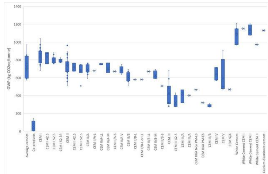
Figure 13. The impact of cements on GWP
