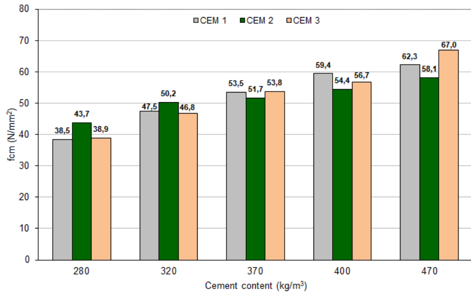
Figure 3. Variation of compressive strengths depending on the cement content, at the age of 90 days
