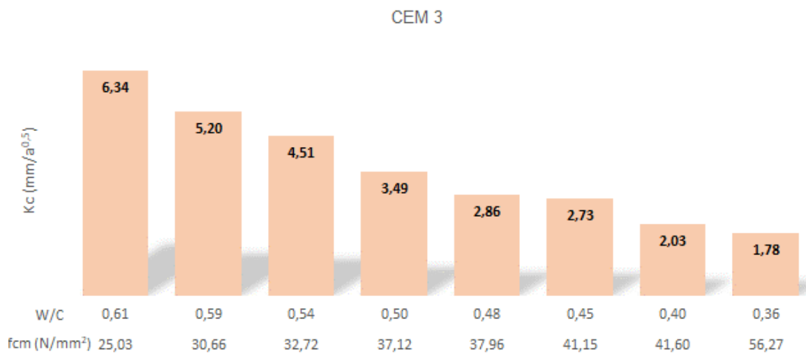
Figure 8. K_c values depending on the W/C ratio and compressive strength at 28 days, for CEM 3
