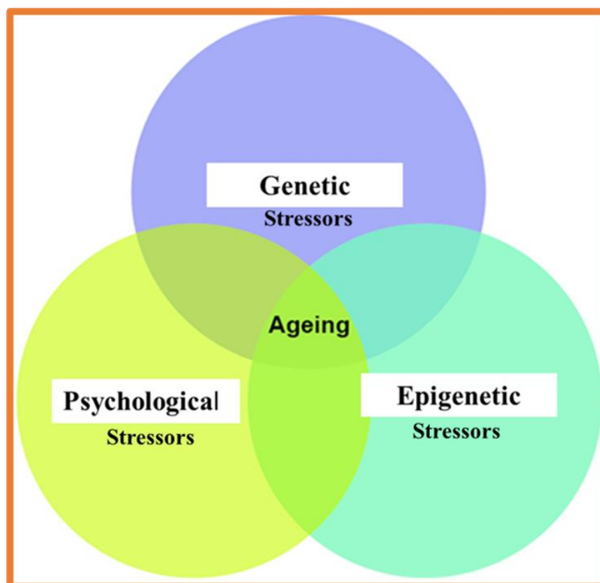
Fig. 2. Major determinant of biological aging.
