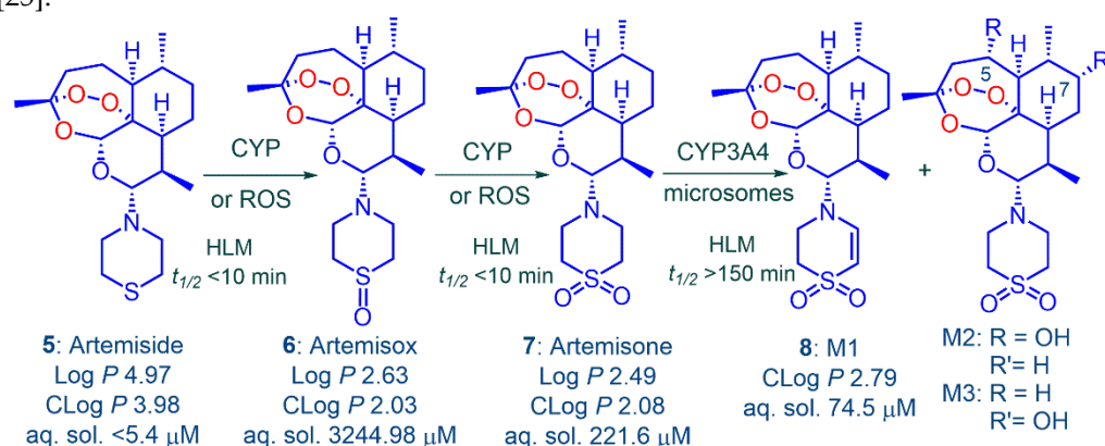
Figure 5. Metabolism of artemiside 5 via enzymatic or non-enzymatic oxidation to artemisox 6 and then to artemisone 7 . Human liver microsomal (HLM) half-lives t_{1/2} for each of artemiside, artemisone and M1 are given [25]. Artemisone is transformed by CYP3A4 into the metabolites M1 8 , M2 and M3, and smaller amounts of other metabolites [24,25,39]. Measured and calculated Log P values (ChemDraw V15.1), aqueous solubility at pH 7.2 for compounds 5-7 are from [24]; aqueous solubility at pH 7.4 for metabolite M1 8 is from [25].
