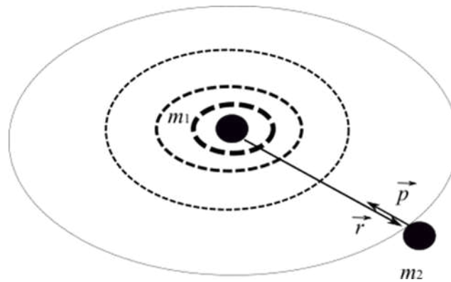
Figure 2. A sketch of a spreading of the circular gravitons in the space. The directions of the spreading rims’ planes are random since in reality any particle is impacted by some forces and isn’t oriented in the space constantly.
