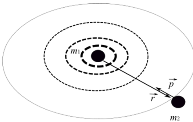
Figure 3. A sketch of a spreading of the circular gravitons in the space. The directions of the spreading rims’ planes are random since in reality any particle is impacted by some forces and isn’t oriented in the space constantly.
