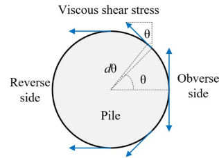
Figure 4. The force analysis of pile foundation.
