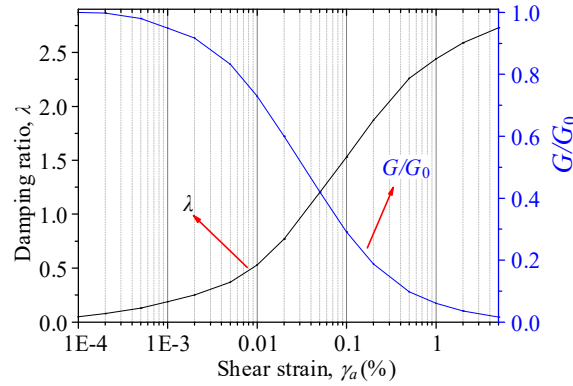
Figure 3. The curves of G/G_{\max} - \gamma_a and \lambda - \gamma_a proposed by Seed and Idriss.
