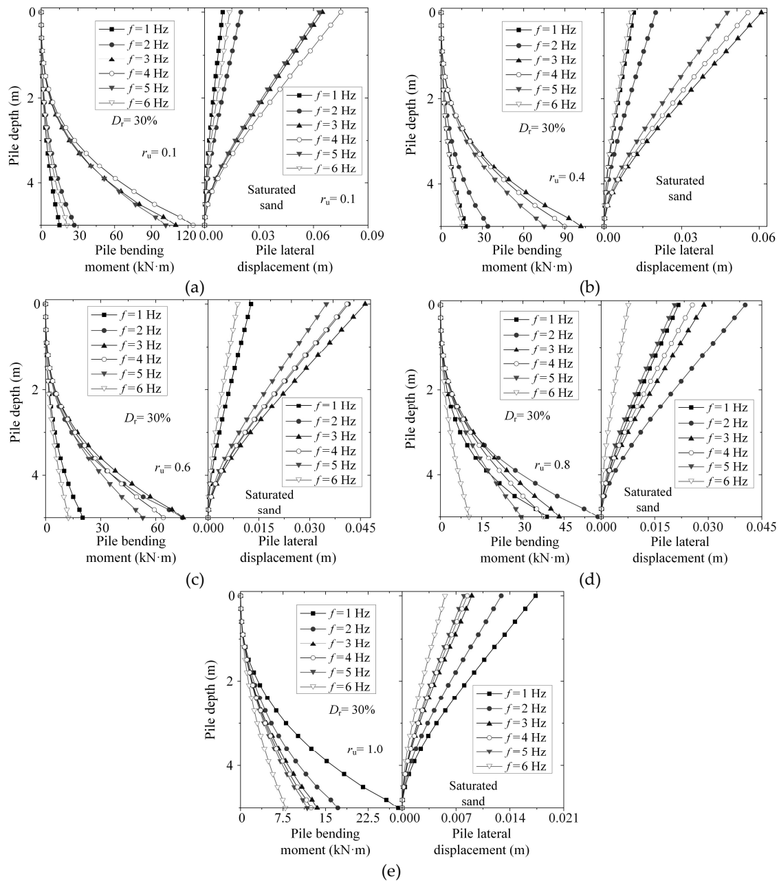
Figure 10. Bending moment and lateral displacement of pile under different loading f : (a) r_u = 0.1 ; (b) r_u = 0.4 ; (c) r_u = 0.6 ; (d) r_u = 0.8 ; (e) r_u = 1.0 .
