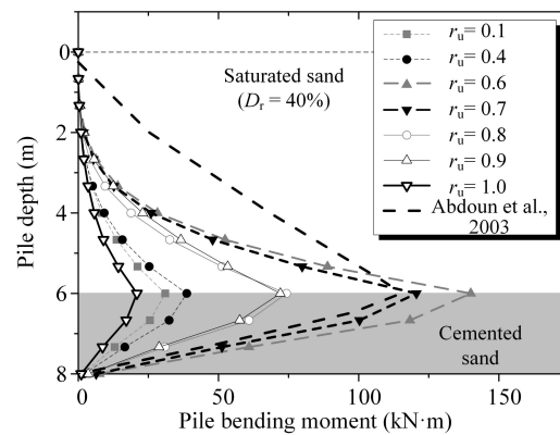
Figure 5. The comparison of computed results and test results.
