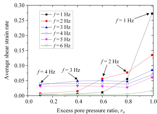
Figure 11. Shear strain rate versus pore pressure ratio for different loading frequency.
