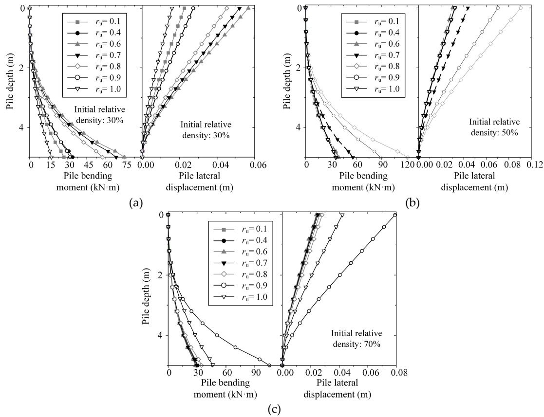
Figure 7. Effect of relative density on pile-soil interaction considering rate-dependent: (a) Relative density of 30%; (b) Relative density of 50%; (c) Relative density of 70%.
