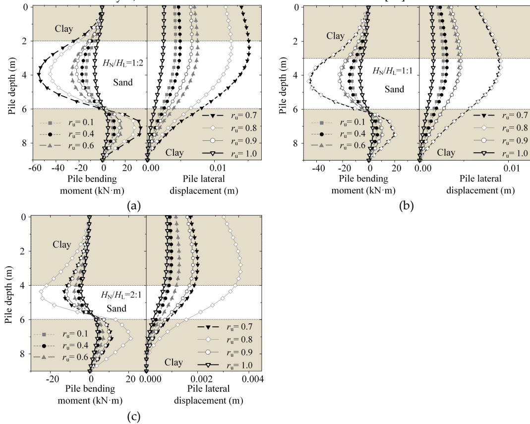
Figure 9. The bending moment and lateral displacement of pile under the foundations with different H_N/H_L : (a) H_N/H_L=1:2 ; (b) H_N/H_L=1:1 ; (c) H_N/H_L=2:1 .
