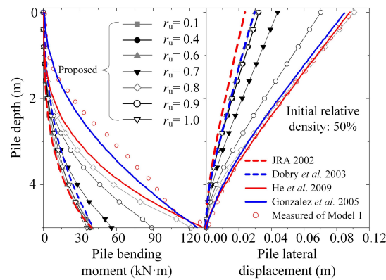
Figure 6. Comparison of pile response obtained using different method.
