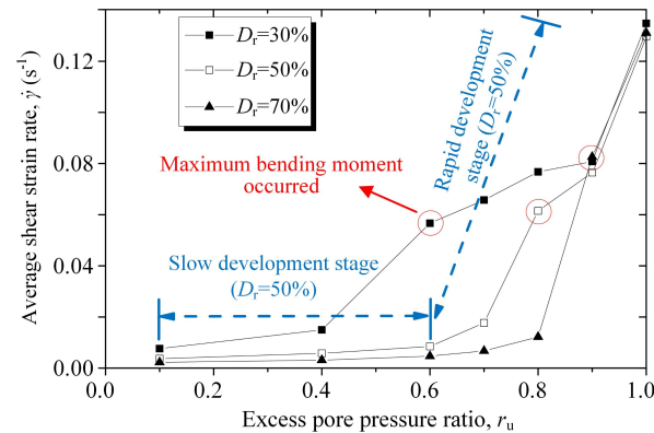
Figure 8. Variation of shear strain rate versus pore pressure ratio for different relative density.
