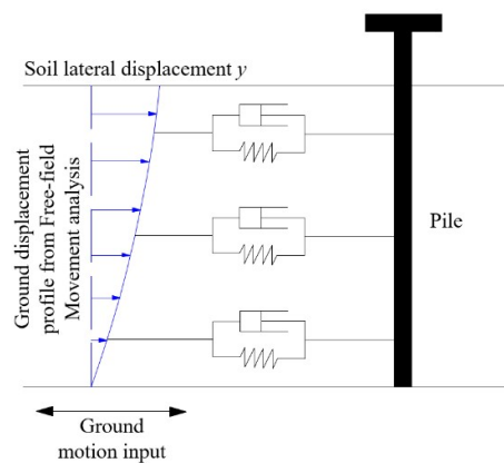
Figure 1. Schematic diagram of p - y curve method.
