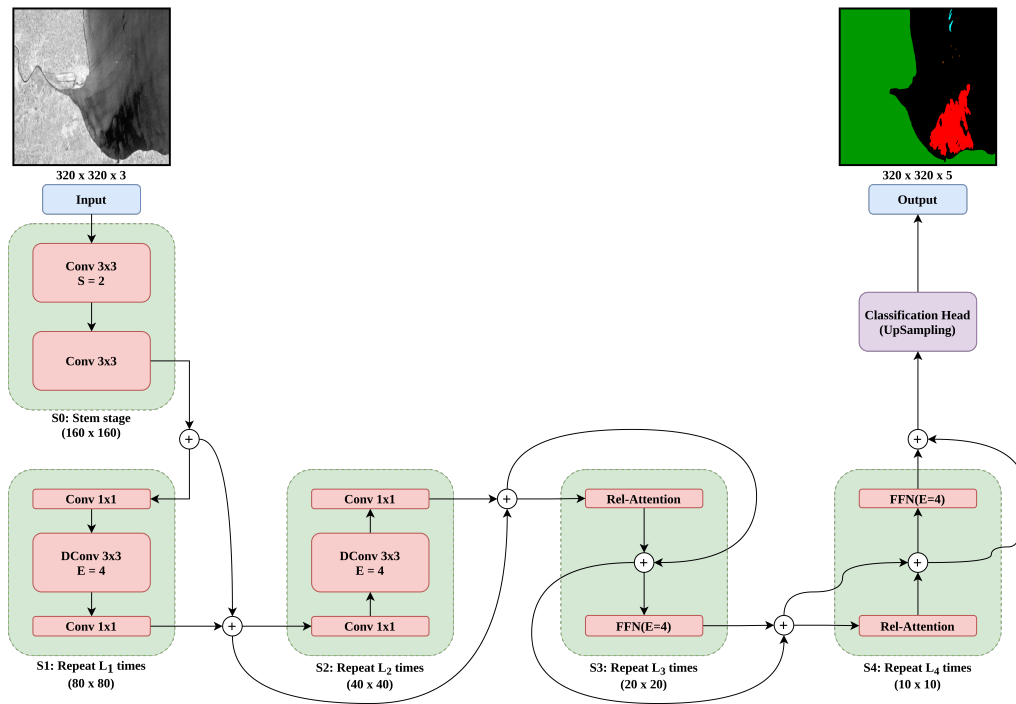
Figure 5. An overview of the CoAtNet architecture used for semantic segmentation of SAR images for oil spill classification. It has five stages, viz., S0, S1, S2, S3 and S4. Each stage reduces the dimensions of the input image by a factor of 1/2. For our classification problem, the input is a 320x320x3 SAR image and output is a 320x320x5 semantic segmentation mask with five desired classes.
