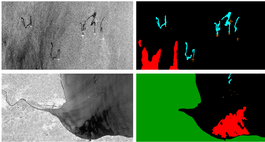
Figure 1. Training dataset: A sample of two Sentinel 1 SAR images ( left ) along with ground truth masks ( right ) and class labels viz. sea surface ( black ), oil spill ( cyan ), look-alikes ( red ), ship ( brown ) and land ( green ). The dataset is prepared by Krestenitis et al. [22] from the MKLab ITI-CERTH, Greece.
