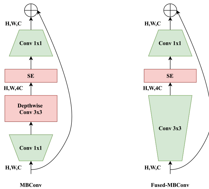
Figure 3. MBConv and Fused-MBConv blocks extensively utilized by EfficientNetV2 CNNs. Fused MBConv blocks are recently proposed for better utilization of mobile or server accelerators. It replaces depth-wise and expansion convolutional layers in MBConv with a single regular convolutional layer. Replacing MBConv with fused-MBConv can improve model training speed with small memory overhead.
