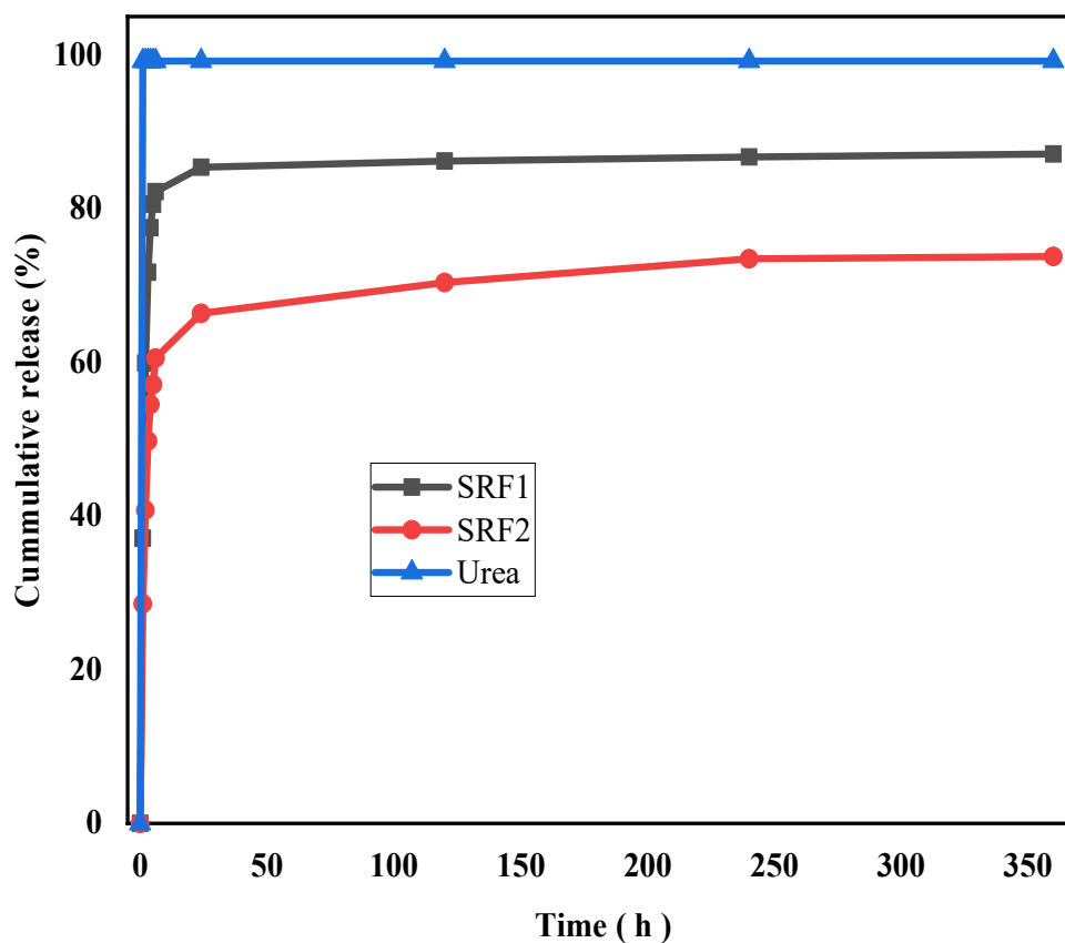
Figure 7: Release Behavior of Urea, SRF1 without Paper and SRF2 with Blended Paper in Water
