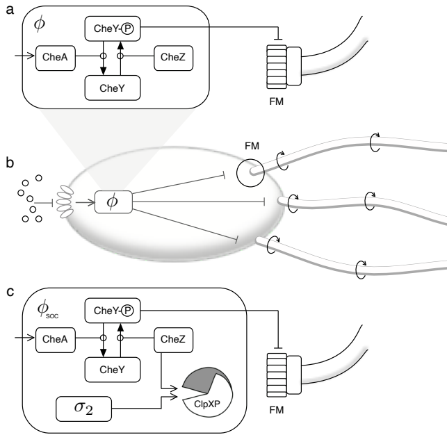
FIG. 5: Using synthetic SOC to modify cell-level search behaviour. A network \phi (a) gathers signals from the environment (such as resources, b) that trigger a response affecting flagellar motor (FM). The \phi network could be expanded into a new one ( \phi_{soc} ) by engineering the degradation of CheZ (c), a key component of this machinery.
