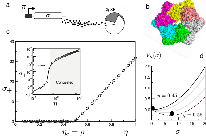
FIG. 2: Free and congested phases in a simple model of queueing dynamics in a genetic circuit. In (a) a single gene is constantly active and produces a protein \sigma at a rate \eta that is also actively degraded by a protease (ClpXP). If production is low, \sigma levels are kept low, but there is a threshold level \eta_c where the degradation machinery becomes overloaded and proteins accumulate, as summarized in (b). (c) The curve of equilibria of model (1) in terms of the rate \eta displays an abrupt transition in the logarithmic scale near \eta = \rho . (d) Associated potential V_\mu(\delta) for different \eta values near the transition point.
