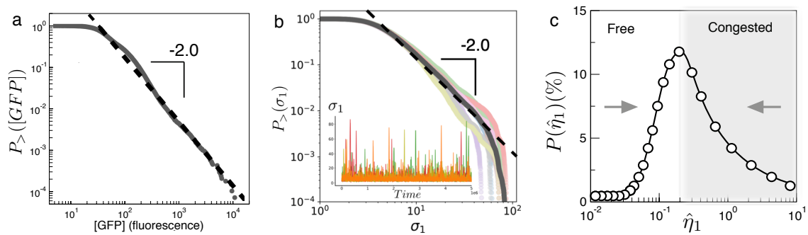
FIG. 4: Statistical patterns of fluctuations of the SOC motif. The experimental (a) and stochastically simulated (b) cumulative distributions consistently reveal a power-law behavior following the same exponent. The inset in (b) shows a time series of \sigma_1 fluctuations. In (c), the self-organized nature of the SOC motif can be visualized by means of the distribution of the effective \eta_1 , here indicated as \hat{\eta}_1 , as defined by equations (12-13). The distribution shows that this quantity peaks at a given value \hat{\eta}_1 \sim 0.02 , close to the mean field result found in the queueing gene model (section 2). The two opposed forces, namely the driving towards higher \sigma_1 expression and the \sigma_2 -mediated repression, are displayed (gray arrows).
