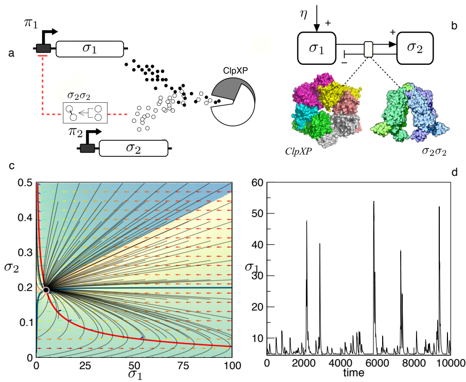
FIG. 3: The SOC genetic motif that generates fat-tailed distributions of protein expression levels. The basic architecture (a) includes two genes whose protein products will play the role of order ( \sigma_1 ) and control ( \sigma_2 ) parameters, respectively. The basic feedbacks between the two are sketched in (b) where two molecular models of the proteolytic machinery (ClpXP) and the inhibitor dimer ( \sigma_2\sigma_2 ) are shown (images generated with Pymol software). In (c) the nullclines and the corresponding vector field of SOC motif is shown for the set \Lambda_0 using \eta_2 = 0.01 . In (d) a time series of \sigma_1 is displayed, with \sigma_2 randomly perturbed in a small amount \sigma_2 = \sigma_2^* - \xi where \xi \in (0, 0.1) with uniform distribution. Bursting dynamics in \sigma_1 are observed.
