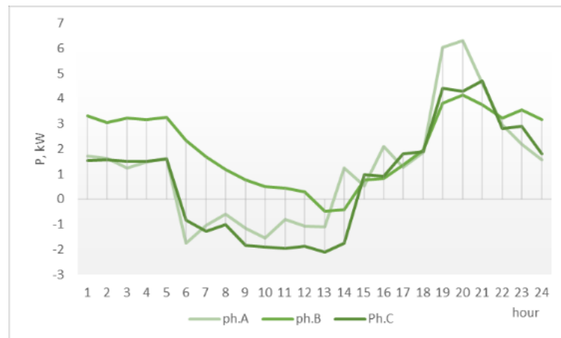
Figure 16. Actual bus demand in network R121 (aggregated demand and generation)
