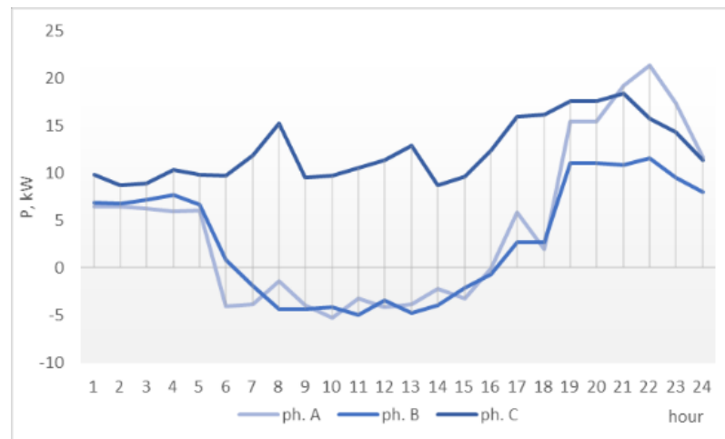
Figure 9. Actual bus demand in network R28 (aggregated demand and generation)
