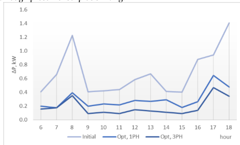
Figure 10. Hourly losses in network R28
