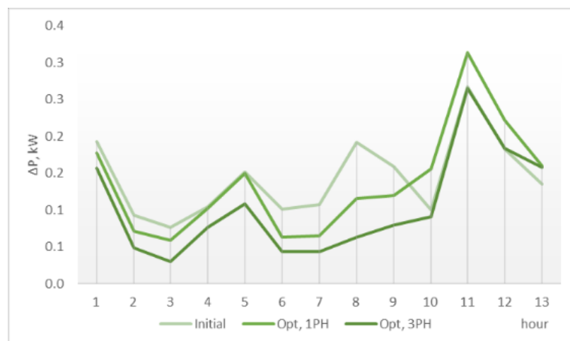
Figure 19. Hourly losses in network R121
