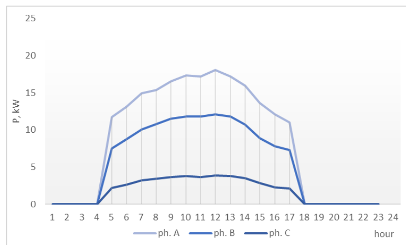
Figure 7. Generation in the network R28
