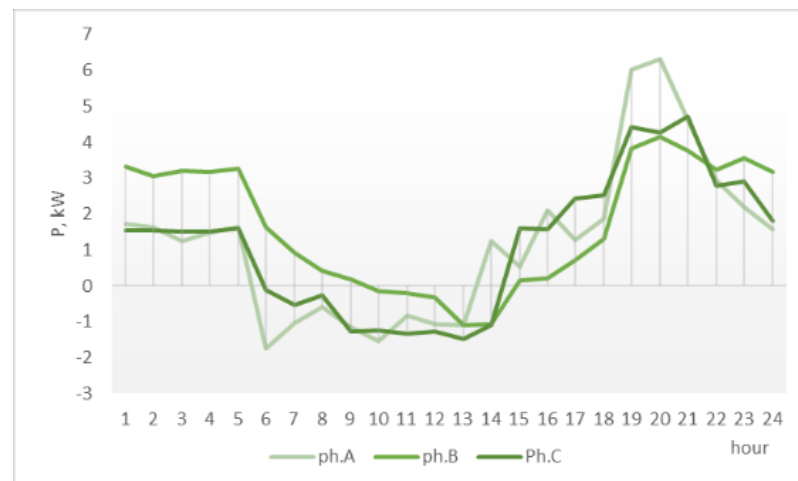
Figure 17. Actual bus demand in network R121 (aggregated demand and generation) – one-phase PSM
