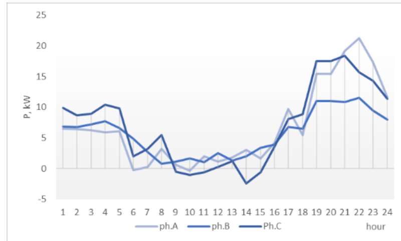
Figure 12. Actual bus demand in network R28 (aggregated demand and generation) – three-phase PSM
