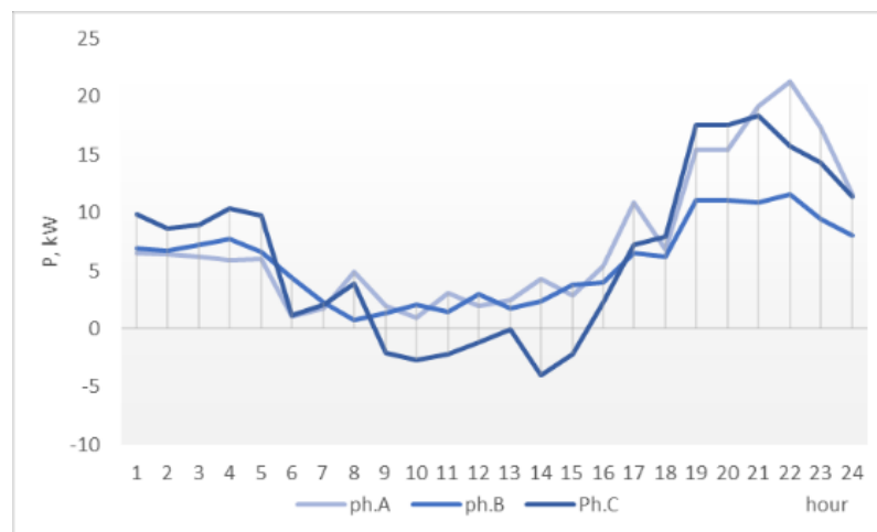
Figure 11. Actual bus demand in network R28 (aggregated demand and generation) – one-phase PSM
