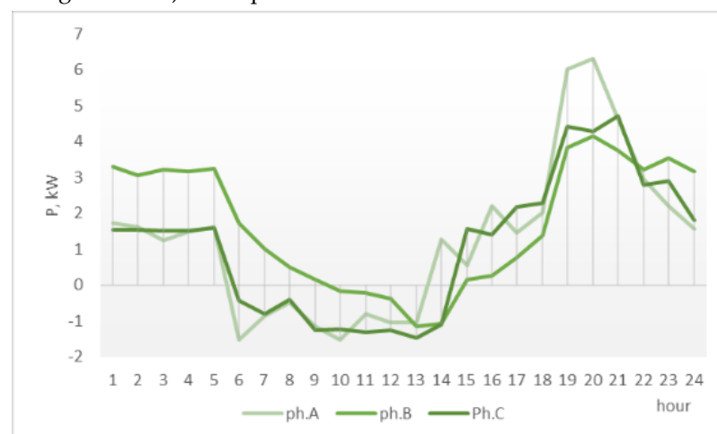
Figure 18. Actual bus demand in network R121 (aggregated demand and generation) – three-phase PSM
