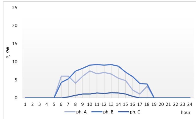
Figure 8. Prosumer surplus in the network R28
