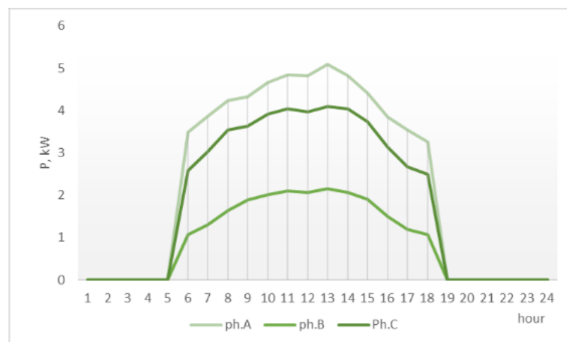
Figure 14. Generation in the network R121
