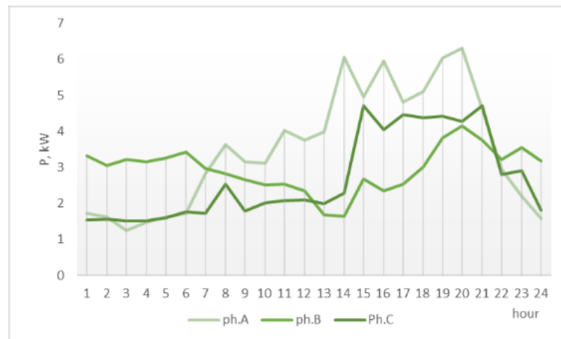
Figure 13. Demand in the network R121
