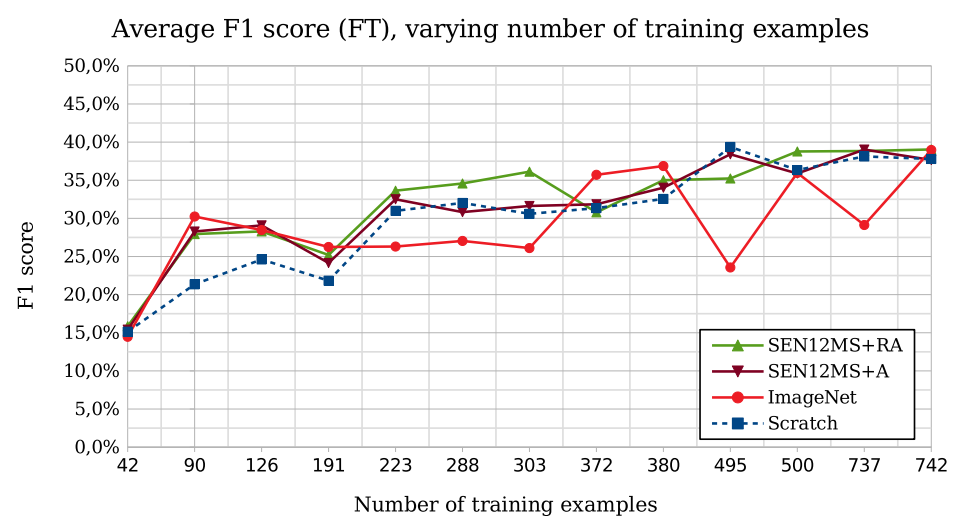
Figure 10. Impact of number of training ships variation on mean F1 score calculated on Brest, Rotterdam and Suez canal
