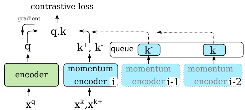
Figure 2. MoCo training algorithm [5]: negative embeddings from momentum encoders at previous iterations ( i-1, i-2 , etc...) are cached and reused at iteration i
