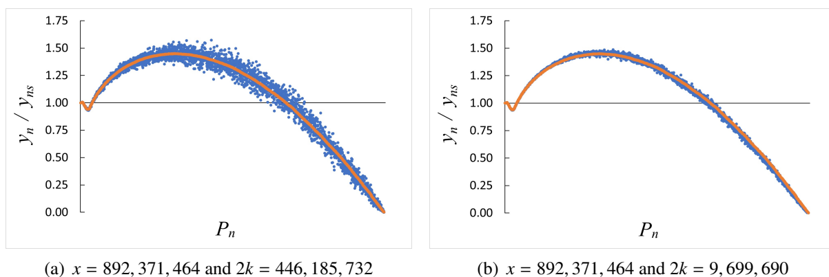
FIGURE 3. \frac{r_n \mathcal{A}_{P_n}}{r_n \mathcal{A}} = \frac{1}{P_n} \cdot y_n (red) and \frac{r_n s\mathcal{A}_{P_n}}{r_n s\mathcal{A}} = \begin{cases} \frac{1}{P_n} \cdot y_{ns}, & \text{if } P_n \mid 2k, \\ \frac{2}{P_n} \cdot y_{ns}, & \text{if } P_n \nmid 2k, \end{cases} (blue).
