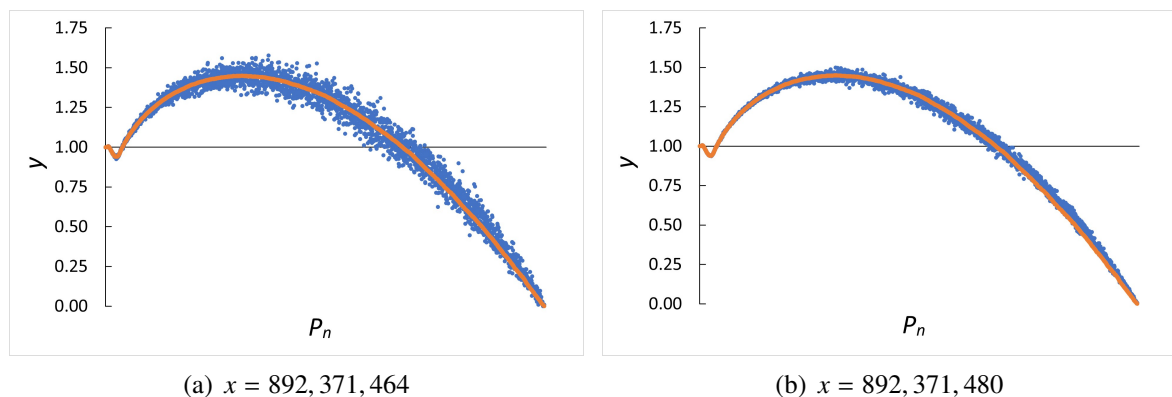
FIGURE 2. \frac{r_n \mathcal{A}_{P_n}}{r_n \mathcal{A}} = \frac{1}{P_n} \cdot y (red) and \frac{r_n a \mathcal{A}_{P_n}}{r_n a \mathcal{A}} = \begin{cases} \frac{1}{P_n} \cdot y, & \text{if } P_n \mid x, \\ \frac{2}{P_n} \cdot y, & \text{if } P_n \nmid x, \end{cases} (blue).
