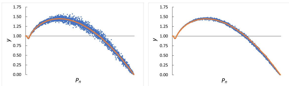
(a) x = 892, 371, 464 and 2k = 446, 185, 732
