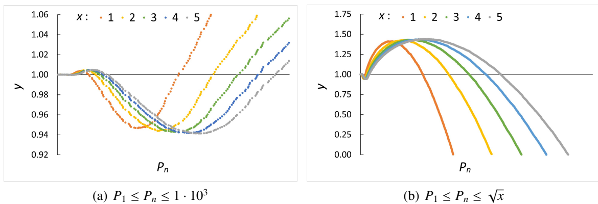
FIGURE 1. \frac{r_n \mathcal{A}_{P_n}}{r_n \mathcal{A}} = \frac{1}{P_n} \cdot y , for various x \cdot 10^8
