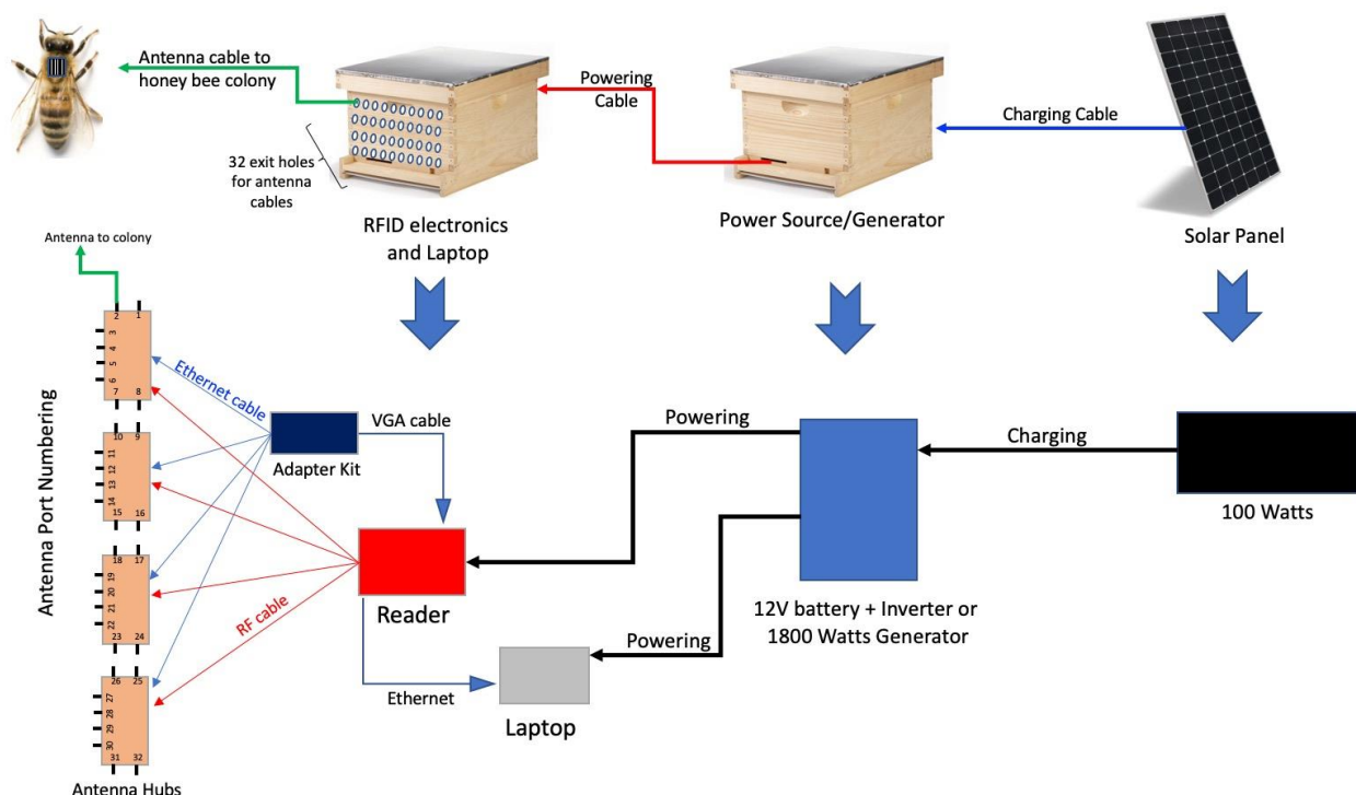
Figure 1. Description of the main operation phases and components of an RFID unit adjusted to accommodate honey bee research. The main items are a power source, RFID reader, portable computer and RFID antenna. Modification of the honey bee hive entrance is required (funnel) to accommodate the antenna.
