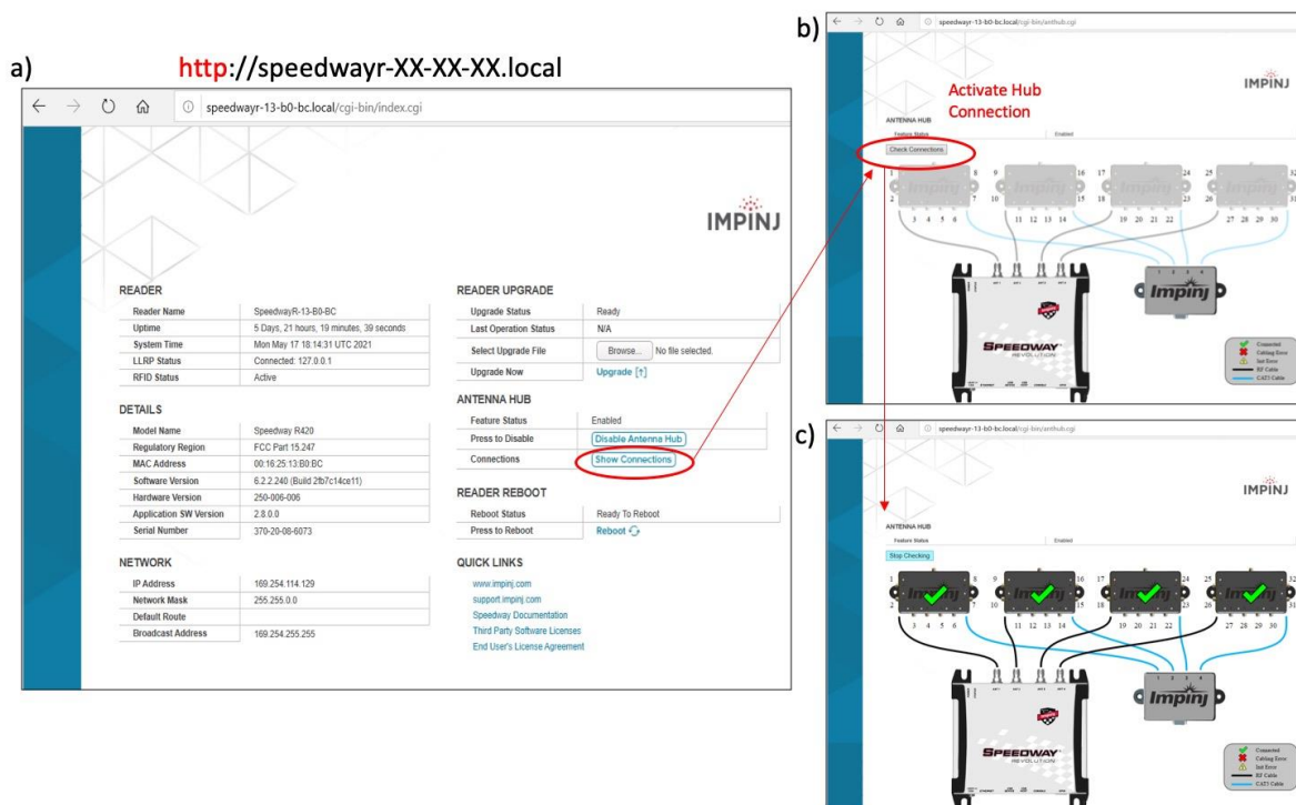
Figure 4. Accessing the primary reader's webpage for parameter changes and activation of connected hubs prior to operating the unit. A) shows the reader webpage address, location where the Speedway Connect software is uploaded, B) interface of hub connectivity and C) confirmation page of all hubs proper connectivity.
