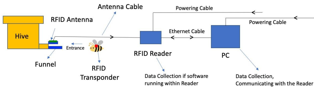
Figure 1. Description of the main operation phases and components of an RFID unit adjusted to accommodate honey bee research. The main items are a power source, RFID reader, portable computer and RFID antenna. Modification of the honey bee hive entrance is required (funnel) to accommodate the antenna.
