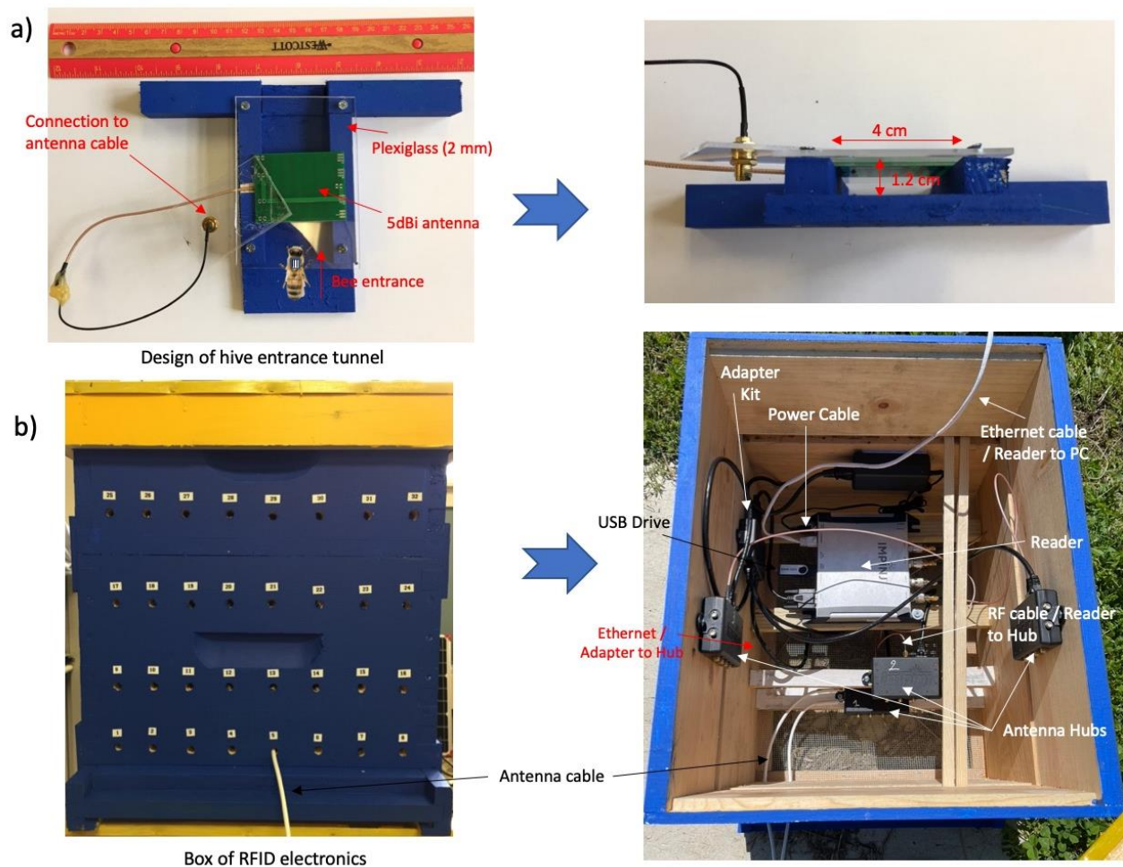
Figure 3. Modification and wiring required to operate the RFID 32-antenna unit. A) shows the optimal tunnel parameters required to accommodate a 5dBi antenna to identify and read the bee's transponder. B) explains the wiring of the various RFID items (reader, hubs and adapter) located within the designated box. For clarity and simplicity, we only displayed the wiring of two antennas.
