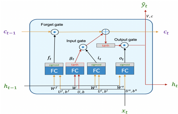
Figure 1. LSTM Structure
