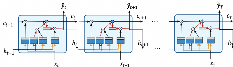
Figure 2. LSTM Overlapping
