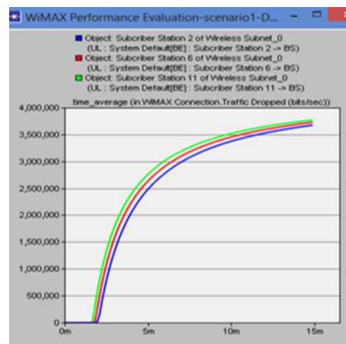
Figure 10. Traffic Dropped
