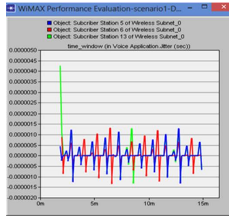
Figure 9. Jitter
