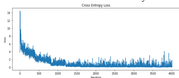
c. Error loss for the dataset with \pm 3 months
