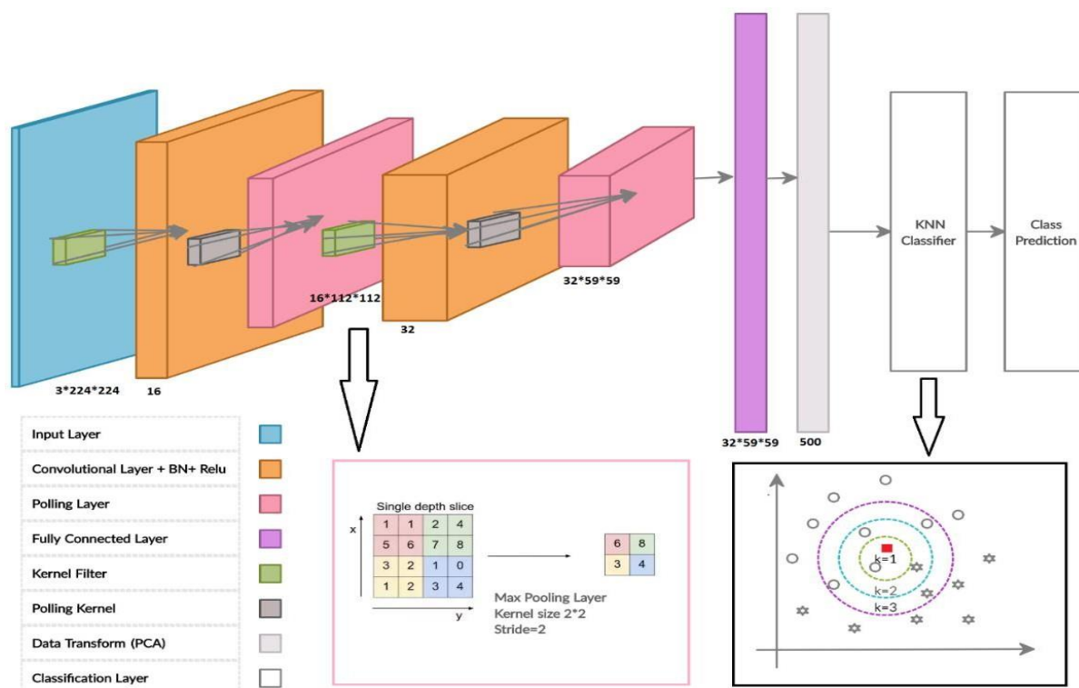
Figure 1. The Architecture of The Proposed HCNN-KNN Model
