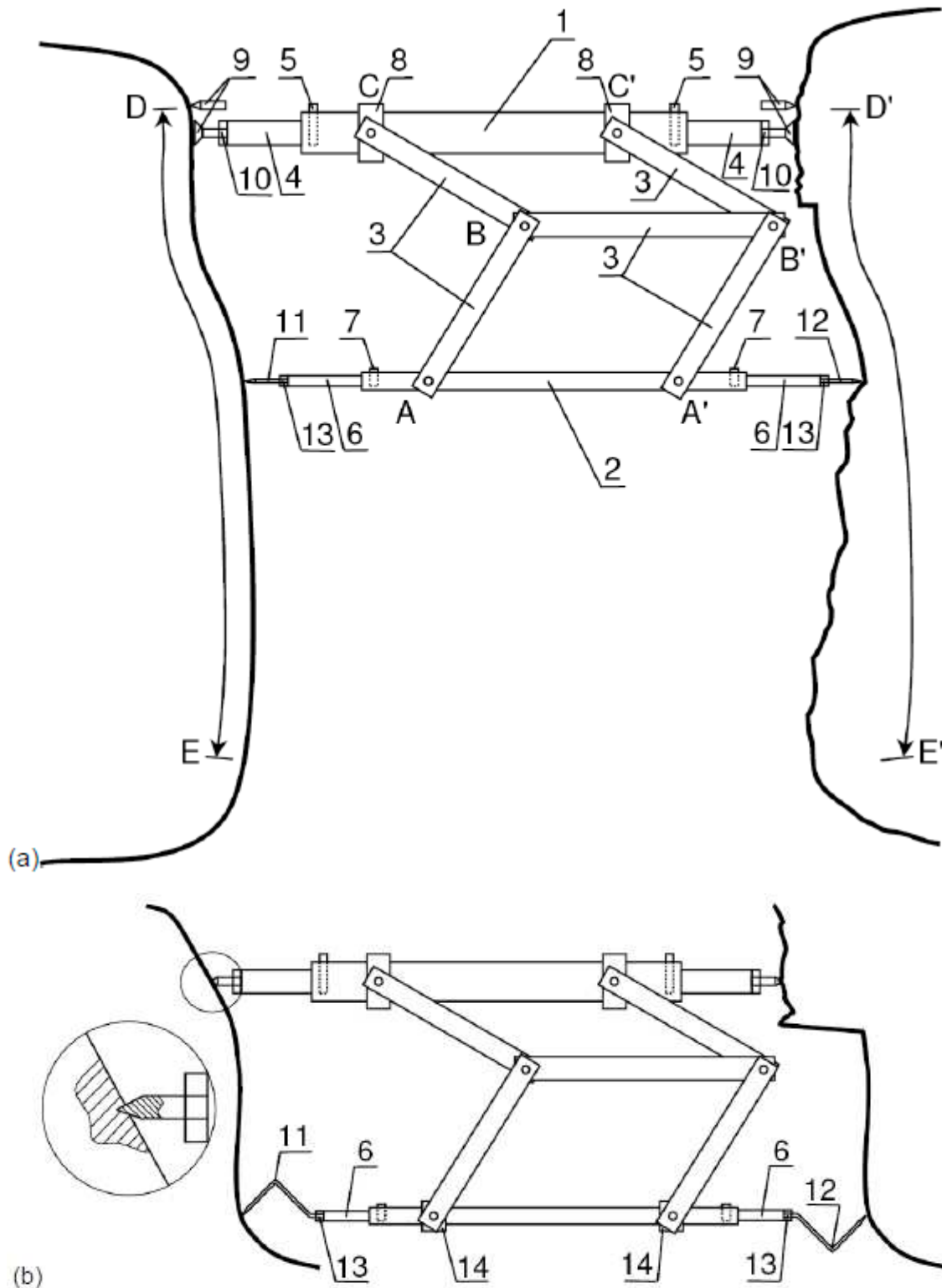
Figure 4. Topography translator: 1 is a carrying rod; 2 is a measuring rod; 3 is a double parallelogram mechanism ( AB=A'B'=BC=B'C' , AA'=BB'=CC' ); 4 are retractable sections for coarse set of length of the carrying rod; 5 are pins locking positions of the retractable sections of the carrying rod; 6 are retractable sections for coarse adjustment of length of the measuring rod; 7 are pins locking positions of the retractable sections of the measuring rod; 8 are cylindrical hinges providing free rotation of the measuring rod along with the double parallelogram mechanism around the carrying rod; 9 are supports (pointed or with a flat foot) of the carrying rod, by unscrewing of which, the carrying rod is set as a strut between two mating stone blocks; 10 are lock-nuts fixing the positions of supports of the carrying rod; 11 is the probe of the measuring rod; 12 is the pointer of the measuring rod; 13 are the
