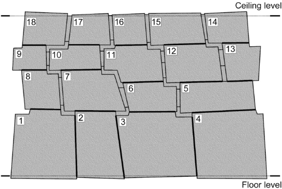
Figure 1. The probable appearance of a casted polygonal masonry of blocks tightly-abutted to each other. The small blocks casted at the final stage are intended for taking up the interblock gaps caused by a concrete shrinkage in the large blocks. The abutment sections between the large blocks (shown with a bold line) are only depicted as rectilinear with zero gaps, in reality, these sections, strictly speaking, are curvilinear and the abutments always have an irregular gap due to the uneven shrinkage. The larger is a shrinkage coefficient and the larger is block sizes, the wider are the gaps. Block deviations from the floor and ceiling levels due to a shrinkage are exaggerated for more clarity. The disadvantage of the masonry is a rather weak bonding of the blocks. The numbers show installation order of the large blocks.
