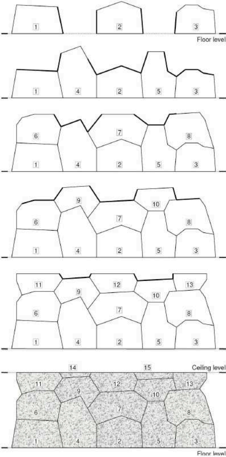
Figure 3. Method of laying of polygonal blocks combining elements of the methods of replica, clay model and 3D-pantograph. The sections, by which the stone blocks are mated at each stage, are shown with a bold line. The numbers designate installation order of the blocks. The interfaces between the blocks are just depicted as rectilinear; in reality, these interfaces are curvilinear in more or less degree.
