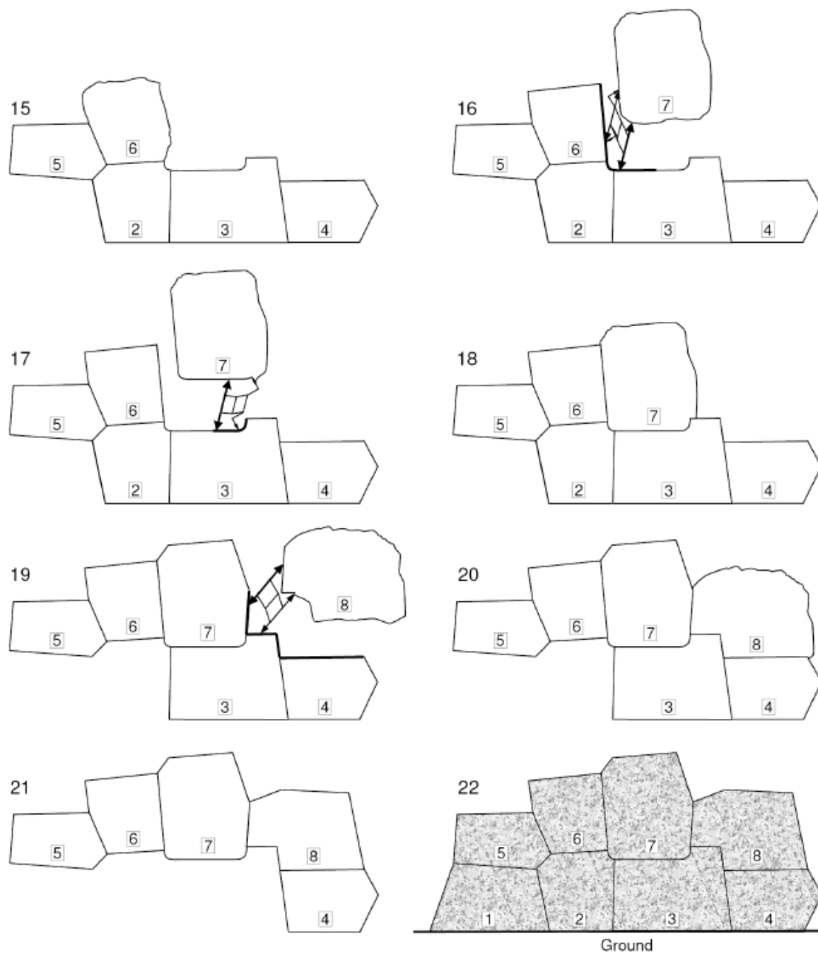
Figure 5. Processing sequence of stone blocks using the topography translator. The polygonal masonry is represented by eight blocks laid in two courses of four blocks in each course. The sections, by which the stone blocks are mated, are shown by a bold line. Except position 22, the stone blocks lie on the ground on their backsides. The translator is shown in a simplified form. Movements of the carrying rod over the processing surface related to the exhaustion of the translator action range are not shown. To transfer the U-shaped recesses, the bent tips are screwed in into the measuring rod instead of the straight ones. The straight-line sections of the interfaces between the blocks are only depicted as straight-line ones; actually, they are curved somewhat.
