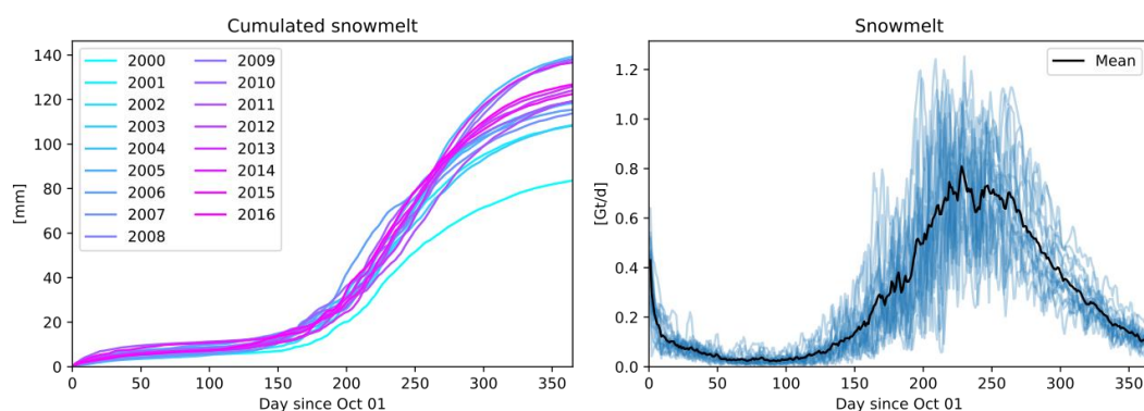
Figure 2. Stacked graphs of cumulated snowmelt and snowmelt timeseries in the Indus basin (the legend indicates the year of the beginning of the water year)
