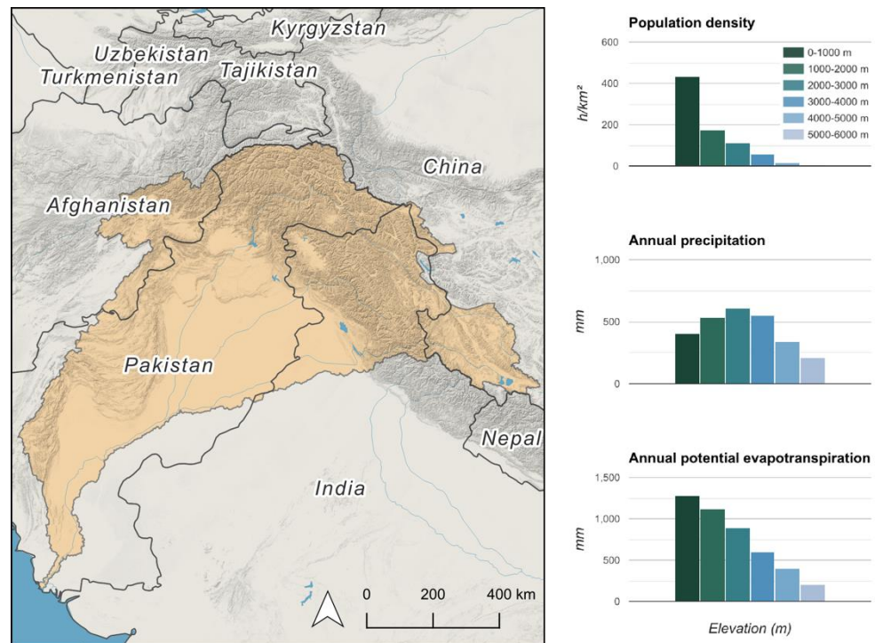
Figure 1. Indus basin map and distribution of population density, annual precipitation and potential evaporation by elevation. Data sources: Global Runoff Data Centre [16] (basin polygon modified in the northeast following [17]), OpenStreetMap (base map), Gridded Population of the World, Version 4 [18], TerraClimate [19].
