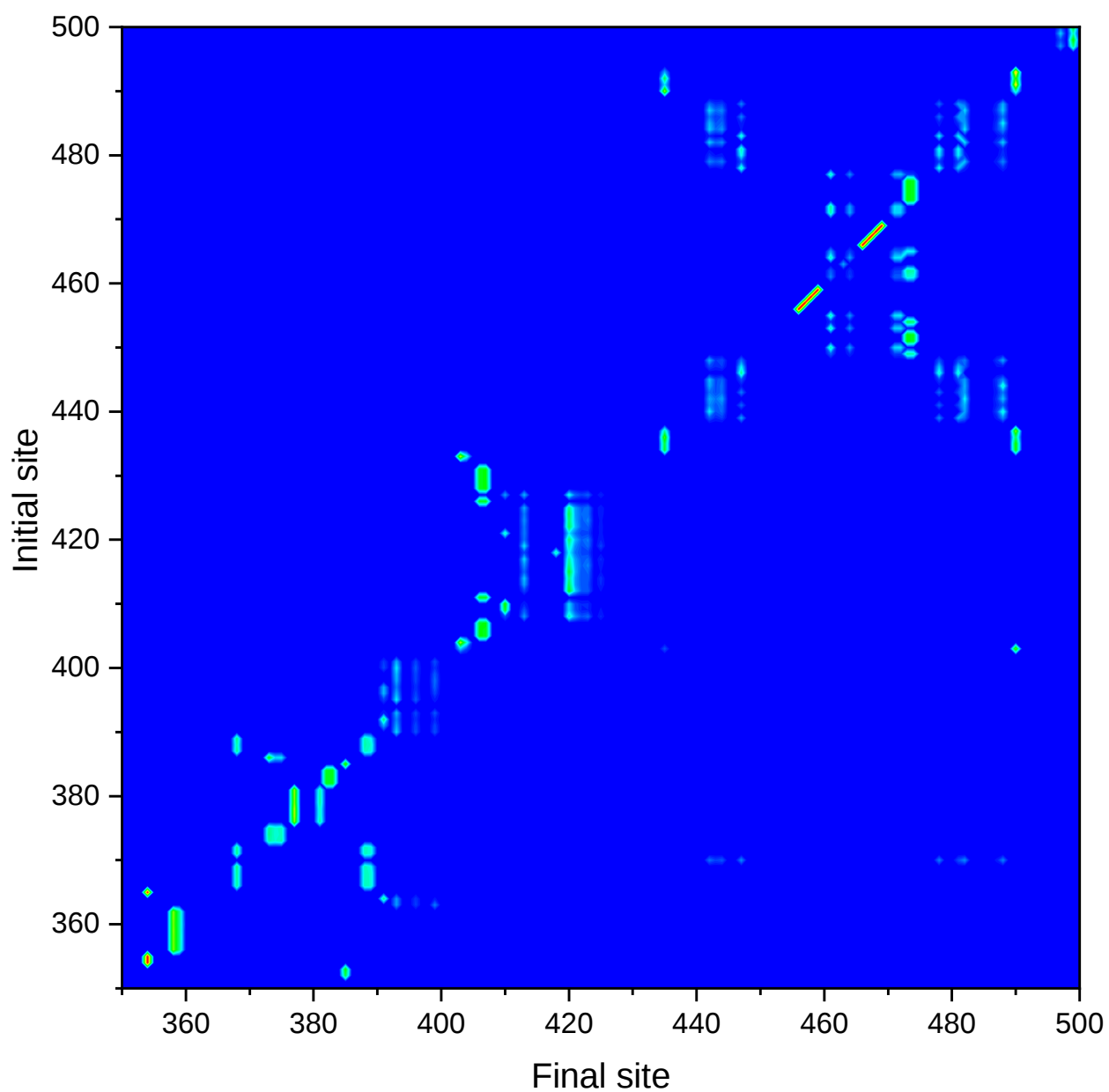
Fig. S3. Transition probabilities map for finding a hole placed at a given initial site at a given final site, in the vicinity of G424.
