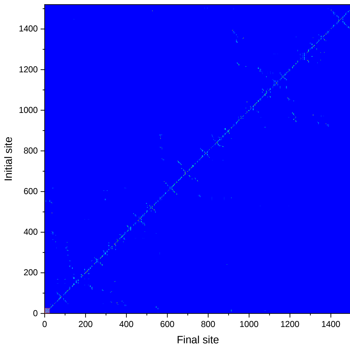
Fig. S2. Transition probabilities map for finding a hole placed at a given initial site at a given final site within SSU.
