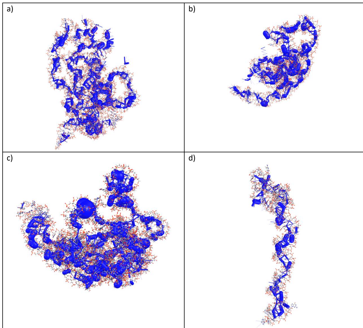
Fig. S1. Charge transfer integrals within 5' (a), central (b). 3' major (c) and 3' minor (d) domains of SSU
