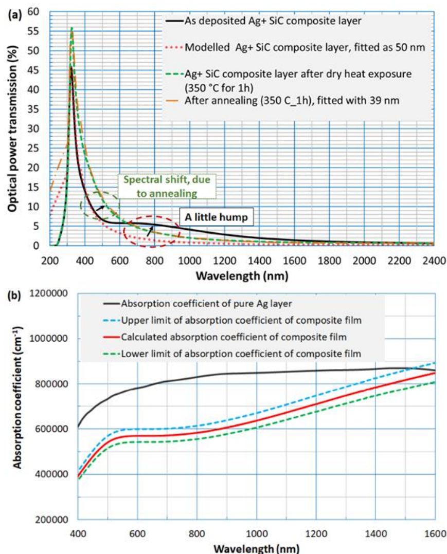
Figure 3. Optical characterization results were obtained from Ag+ SiC thin-film nanocomposite layers.
