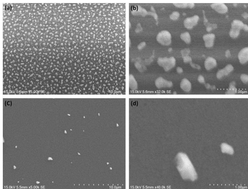
Figure 4. Morphological study of heat-treated pure-Ag and Ag + SiC (5 vol. %) composite layers. SEM images of Ag thin layer were obtained after annealing at 350 °C for 1 h (a, b) and, Ag + SiC composite thin layer was imaged after exposure to the same temperature (350 °C for 1 h) (c, d). Surface imperfections in images (c) and (d) may be due to surface contamination, or slight precipitation.
