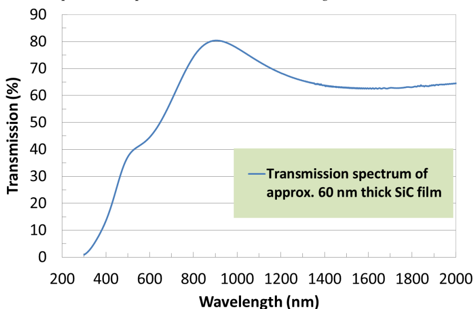
Figure 2. Optical transmission spectrum of an amorphous SiC layer prepared by using RF magnetron sputtering technique.
