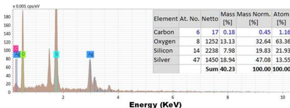
Figure 5. Elemental study of Ag + SiC (5 vol. %) composite layer.
