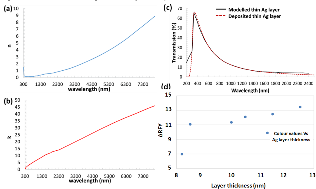
Figure 1. Extrapolated digitized optical constants dispersion data (a b), Optical (c) [32], and the color (d) characterization results for thin sputtered Ag layers. The color values (measured using
