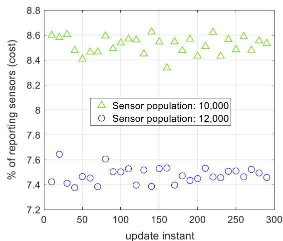
Figure 8. The percentage of reporting sensors to the FC for two different sensor populations. The number of reporting sensors does not tangibly change, when the sensor population changes.
