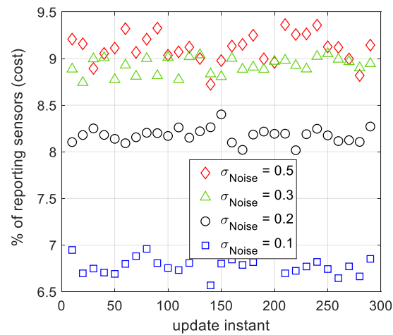
Figure 7. The tracking cost of SSG for several filtered observation noise strengths, during several tracking instances. The sensors apply moving average filter on their local observations to reduce the effect of additive noise.
