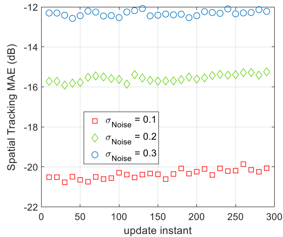
Figure 9. The spatial tracking MAE of AWSG at different observation noise's strength. As the standard deviation of the observation noise increases, the modeling performance drops.
