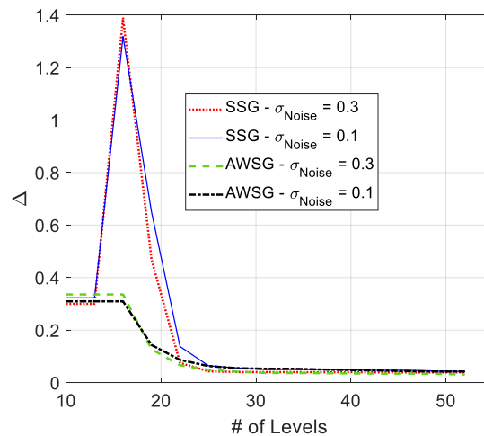
Figure 10. Variation of \Delta in the course of convergence in SSG and AWSG in the presence of filtered observation noise.
