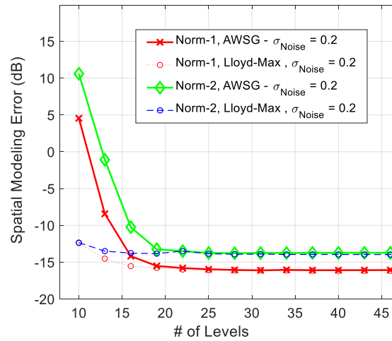
Figure 5. Comparison between the spatial modeling error of norm-1 (MAE) and norm-2 (RMSE) in convergence process of AWSG.
