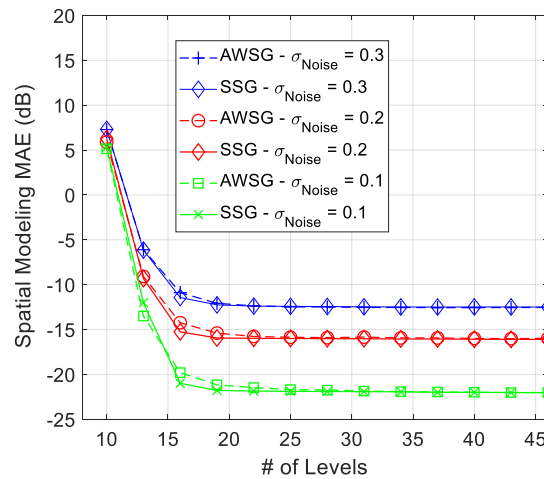
Figure 4. Comparison between the convergence speed of AWSG and SSG, during convergence process of the algorithm.
