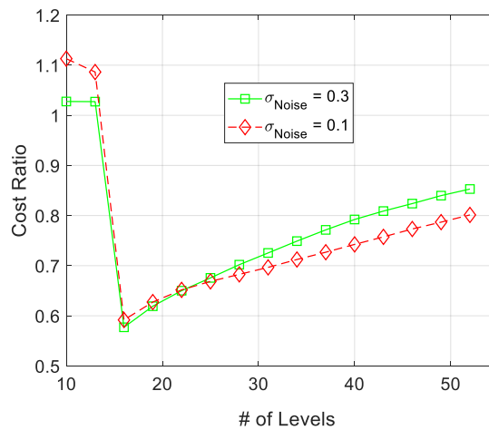
Figure 6. Comparison between the spatial modeling cost of AWSG and SSG. The relative cost R = Cost_{SSG}(k)/Cost_{AWSG}(k) is sketched for two different filtered noise strength in sensor observations.
