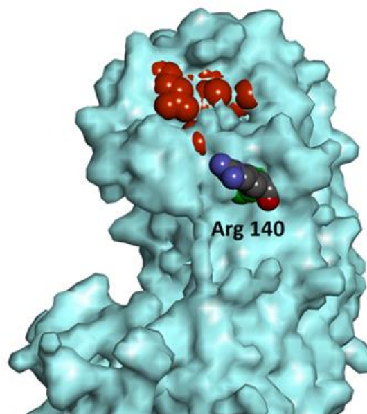
Figure 1. Arg140 location near the hemagglutinin receptor binding site. Atomic coordinates of H7 HA (1ti8) were used [24]. The protein surface is colored blue. The key amino acids of receptor binding site are colored red. The Arg140 colored by element.
