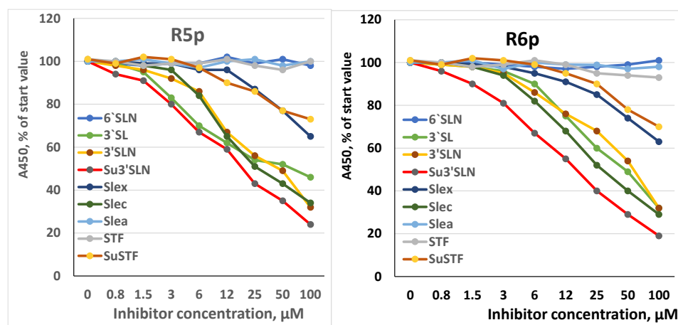
Figure 5. Inhibition of labeled fetuin binding to R5p and R6p viruses by the receptor analogs. Receptor analogs were added to a solution of labeled fetuin at the indicated concentrations and the level of binding of the label to the virus was measured. Result of a typical experiment is presented.
