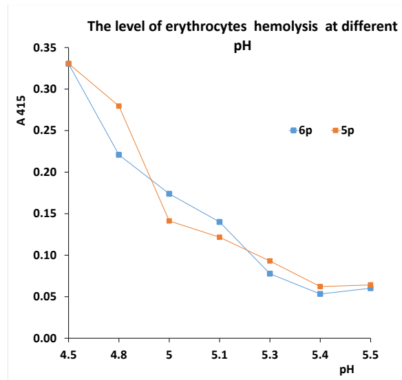
Figure 3. The pH dependence of erythrocyte hemolysis in complex with R5p and R6p viruses. A_{415} - absorption at 415 nm, which corresponds to the degree of erythrocyte hemolysis. Result of a typical experiment is presented.
