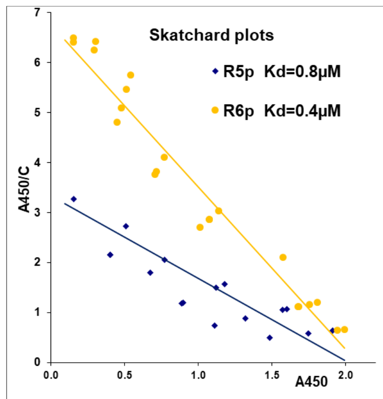
Figure 4. Affinity of peroxidase labeled fetuin for virions of R5p and R6p strains. The results of testing Fet-HRP on a plate coated with R5p and R6p viruses are presented in Scatchard coordinates. The X-axis is the A_{450} signal reflecting the amount of bound fetuin, and the Y-axis is the ratio of the A_{450} signal to the fetuin concentration (expressed in \mu\text{M} of sialic acid) in the solution. Result of a typical experiment is presented.
