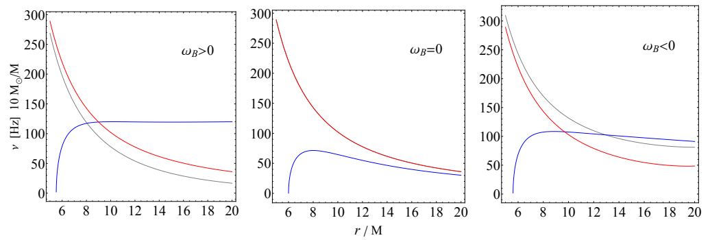
Figure 4. Radial dependence of the fundamental frequencies for for positive \omega_B > 0 , zero \omega_B = 0 and negative \omega_B < 0 values of the interaction parameter. The gray line represents Keplerian frequency, while the blue and red lines are responsible frequencies for the radial and vertical oscillations.
