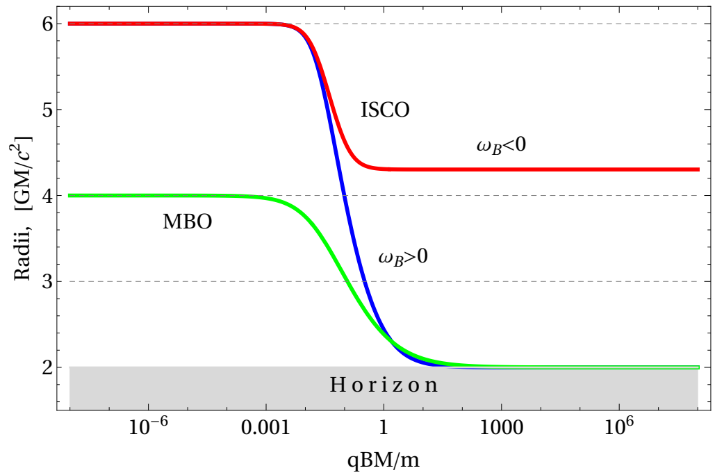
Figure 1. Dependence the ISCO and MBO radii from the magnetic coupling parameter qBM/m for the positivle and negatively charged particle.
