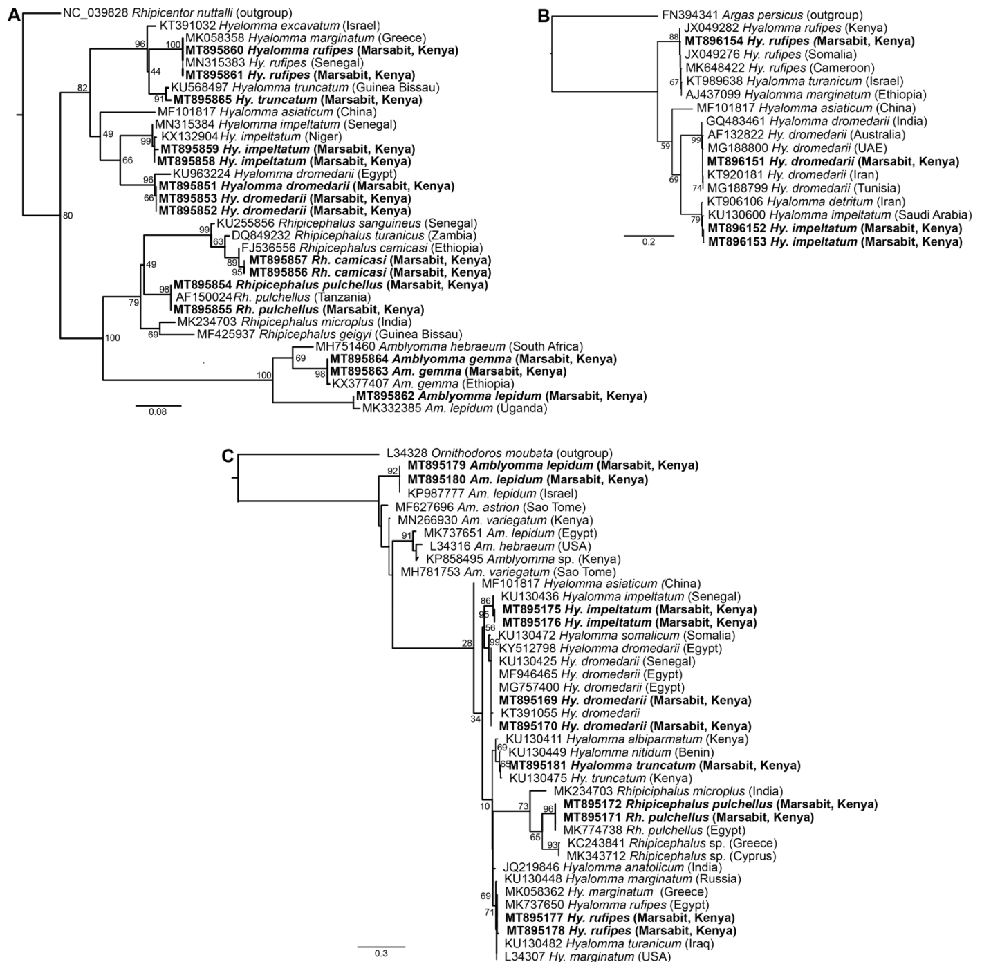
Figure 3. Maximum likelihood phylogenetic trees of representative gene sequences from samples of ticks collected from camels in Northern Kenya. (A) 12S rRNA, (B) COI mitochondrial and (C) 16S rRNA gene sequences. Sequences obtained from this study, with their GenBank accession numbers, are in bold. Bootstrap values at the major nodes are of percentage agreement among 1000 bootstrap replicates. The branch length scale represents substitutions per site. Trees are rooted to outgroup sequences (indicated in brackets; top sequence of each tree).
