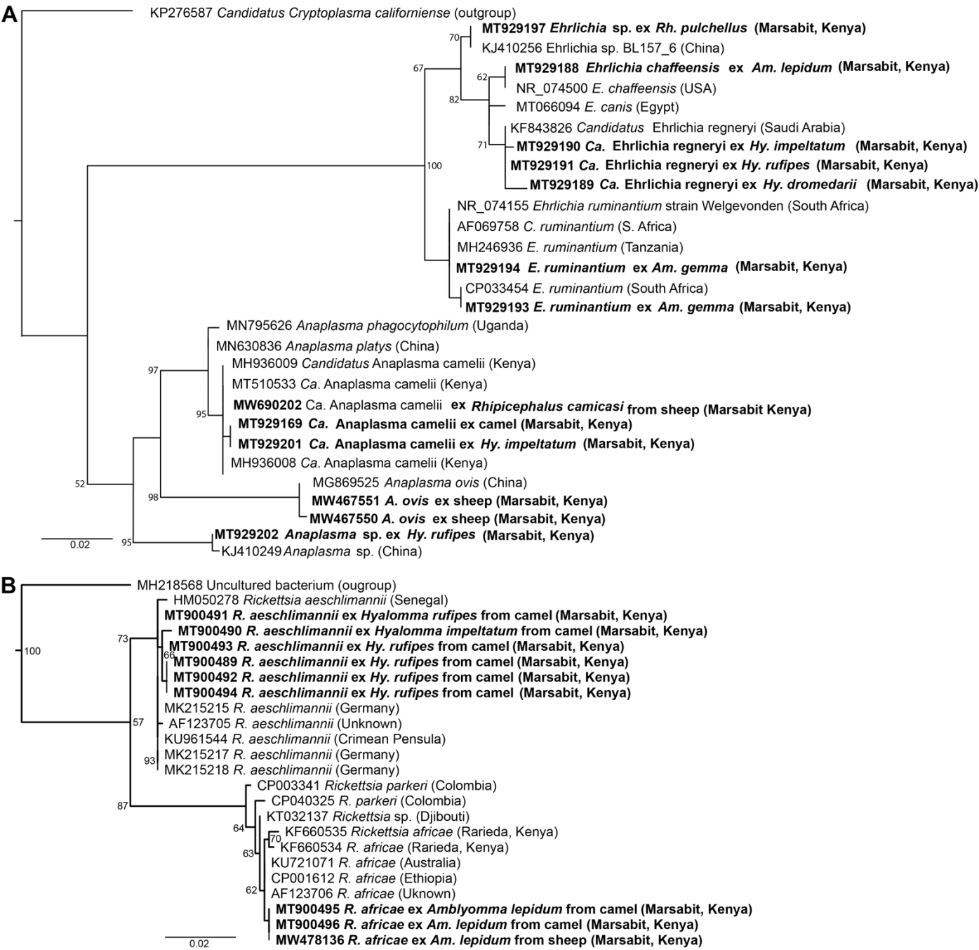
Figure 5. Maximum likelihood phylogenetic trees of A) 1030-bp Anaplasma spp. and 451-bp Ehrlichia spp. 16S rRNA sequences, and B) 857-bp Rickettsia spp. ompB sequences. Sequences amplified from blood and ticks infesting camels in northern Kenya in this study are indicated in bold. Bootstrap values at the major nodes are of percentage agreement among 1,000 bootstrap replicates. The branch length scale represents substitutions per site. Trees are rooted to out-group sequences (indicated in brackets; top sequence of each tree).
