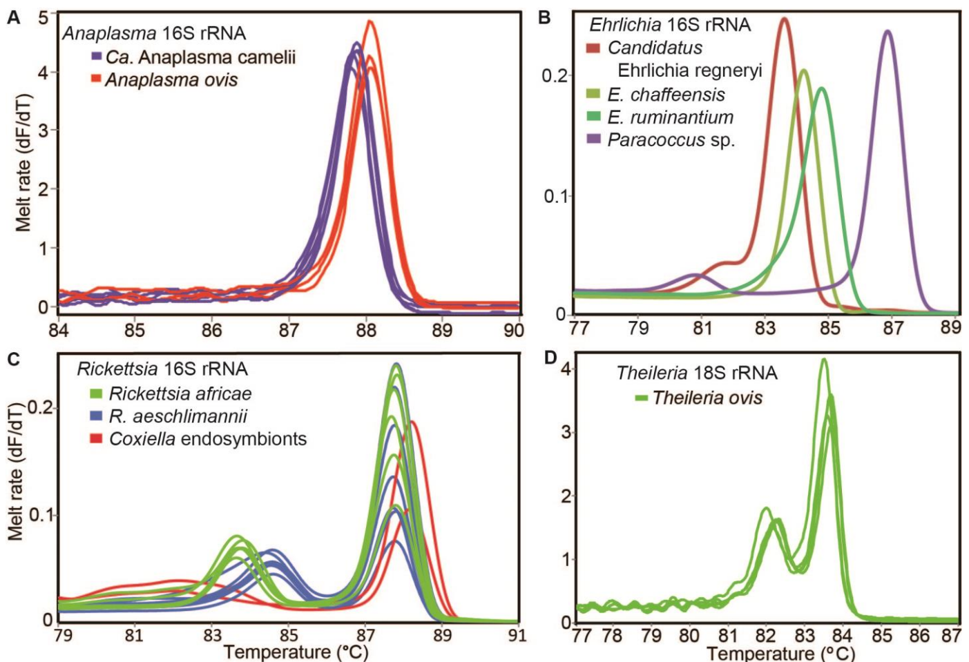
Figure 4: Representative melt rate profiles of tick-borne pathogens in tick samples collected from camels and sheep in northern Kenya. PCR-amplicon melt rates are represented as change in fluorescence with increasing temperature (dF/dT) of (A) Anaplasma 16S rRNA, (B) Ehrlichia 16S rRNA, (C) Rickettsia 16S rRNA and (D) Theileria 18S rRNA gene amplicons.
