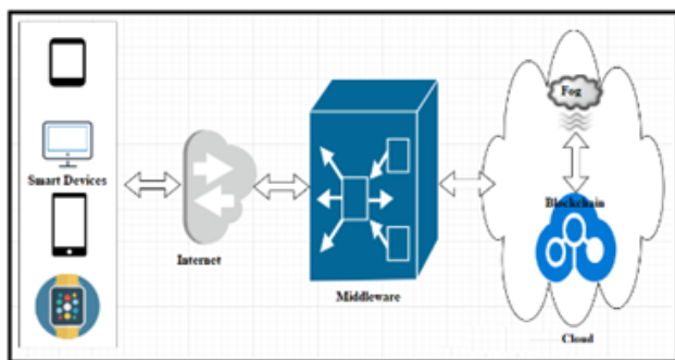
FIGURE 1. IoT-Fog Framework
