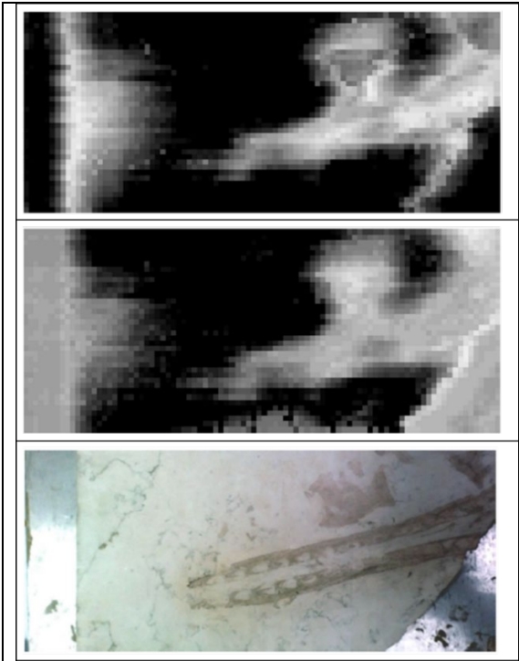
Fig. 35 Summed modulus of parallel and cross polarization scans at 6.7 GHz (top); summed modulus of scans 6.4 GHz, 6.5 GHz, 6.6 GHz and 6.7 GHz parallel and cross polarizations (middle); photograph of the lower side of the limestone slab aligned to correspond with the scanned area (bottom).
