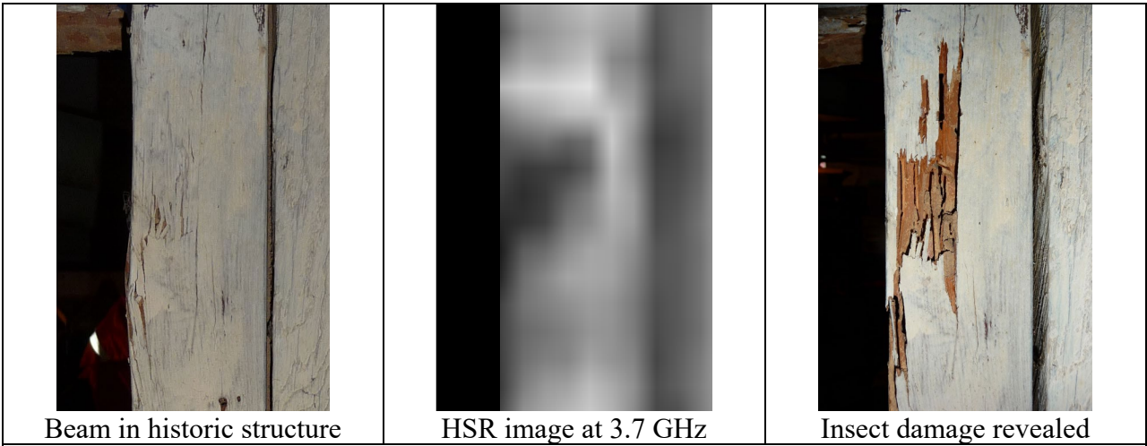
Fig. 32 Wooden beam in historic structure with insect damage detected and revealed.
