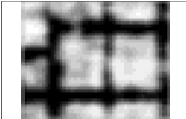
Fig. 8 Radar image of reinforcing in concrete at 3.9 GHz. Mesh spacing is 20 cm x 20 cm at a depth of 3 cm to 4 cm [39].
