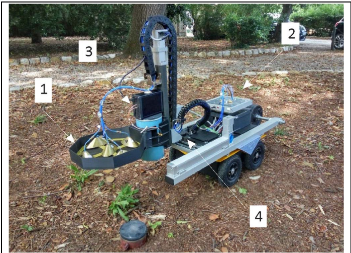
Fig. 20 Robotic platform “Ugo 1st” [89]; 1)ISR antenna array, 2) ISR controller, 3) HSR, 4) 3-D camera.
