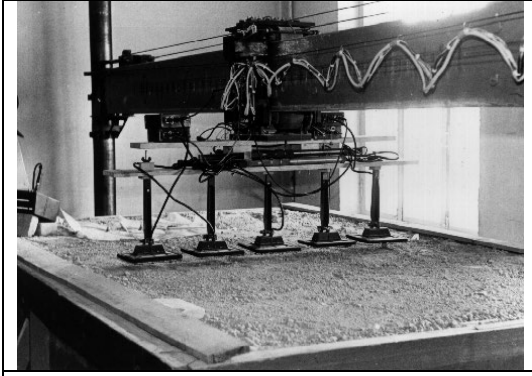
Fig. 12 Mock-up of a wide-span system for mine detection.
