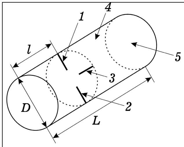
Fig. 7 Design of holographic subsurface radar antenna [59]. The drawing shows the main elements of the design as described in the following: (1) emitting feed antenna, (2) receiver feed antenna for parallel polarization, (3) receiver feed antenna for cross polarization, (4) round waveguide, (5) open end of waveguide. The following dimensional parameters are: D – waveguide diameter, L – waveguide length, l – distance between closed end of waveguide and plane of pin antennas 1 and 2.
