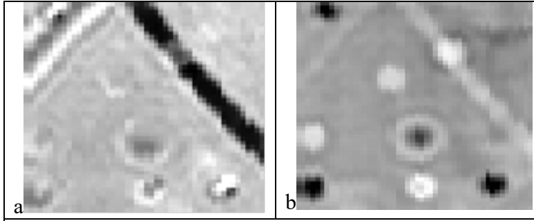
Fig. 9 Cross a) and parallel b) polarization received signals recorded at frequency of 4.0 GHz [39]. These images were recorded for a test wall inside of which small coins and metal wires were placed at different depths.
