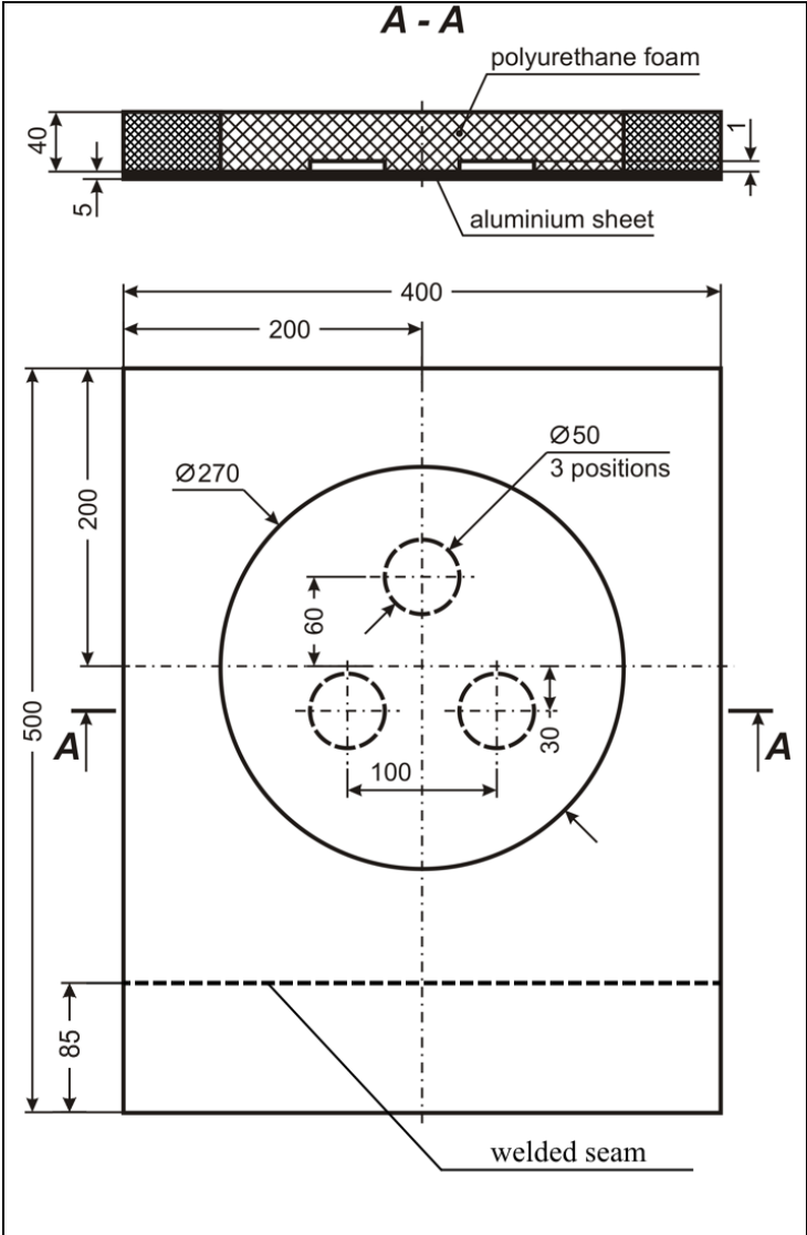
Fig. 24 Mechanical drawing of composite mock insulation with three artificial defects.
