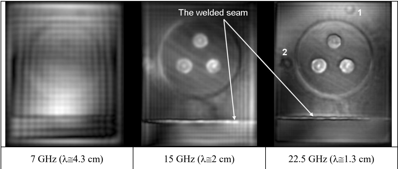
Fig. 25 HSR images of the aerospace materials test sample with intentional (and unintentional) defects.
