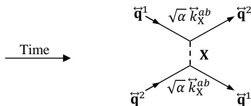
Crossbred dead-end bosons interactions
