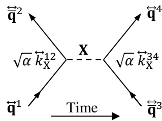
Crossbreed fermions annihilation & creation (3.3-2)
