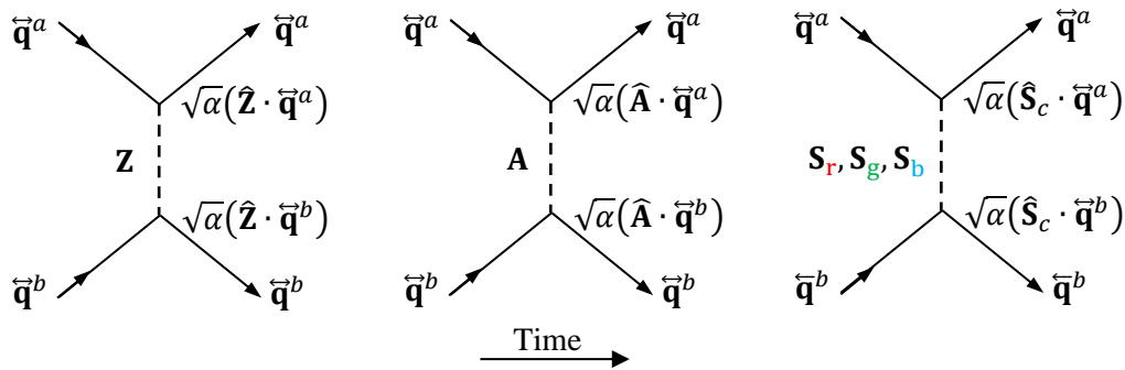
Fermions interacting by “exchanging” Z , A and S c potential bosons (3.2-7)
