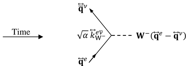
Electron/Anti-neutrino annihilation (3.3-8)
