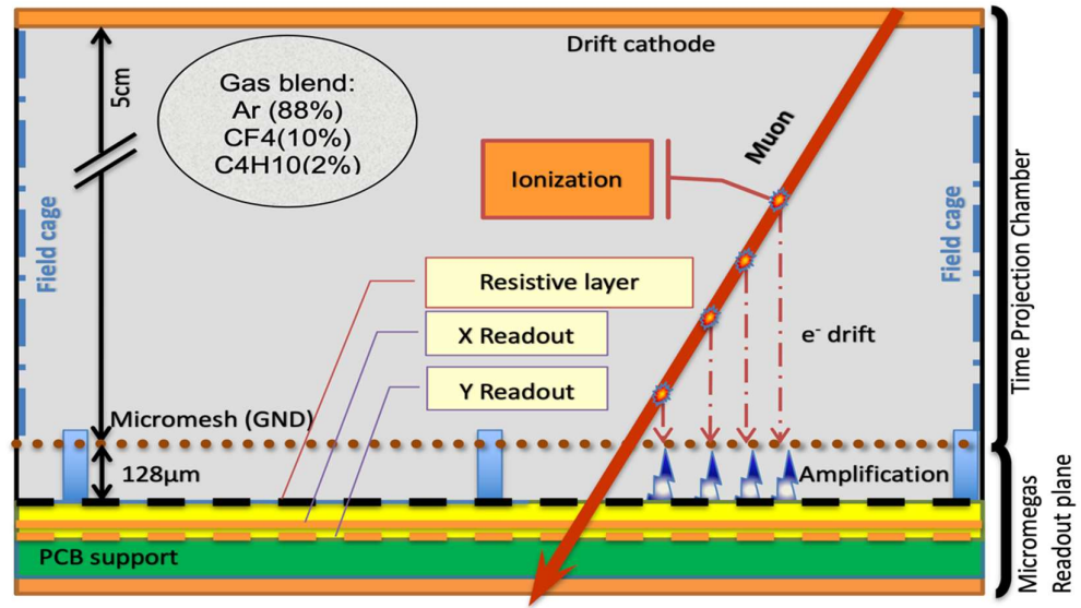
Figure 1. Schematic cross-section of the MUST 2 detector to illustrate its working principle. Figure from [10].
