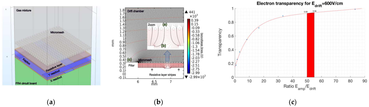
Figure 3. (a) Schematic representation of the unit cell of the MUST 2 detector for transparency simulations. (b) Electrostatic simulation near the micromesh. (c) Results of transparency simulations as a function of the \vec{E}_{amp}/\vec{E}_{drift} ratio.
