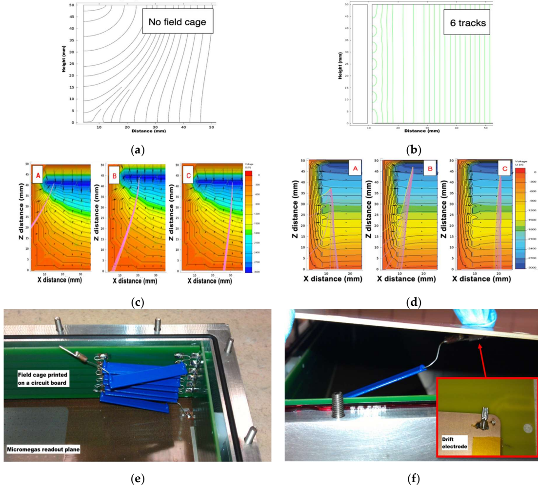
Figure 2. Representation of the field lines within the drift volume without (a) and with (b) the field cage. Simulation of the electron drift path (pink lines) inside the TPC without (c) and with (d) field cage. (e) Inner view of the TPC and (f) connection to the drift electrode.
