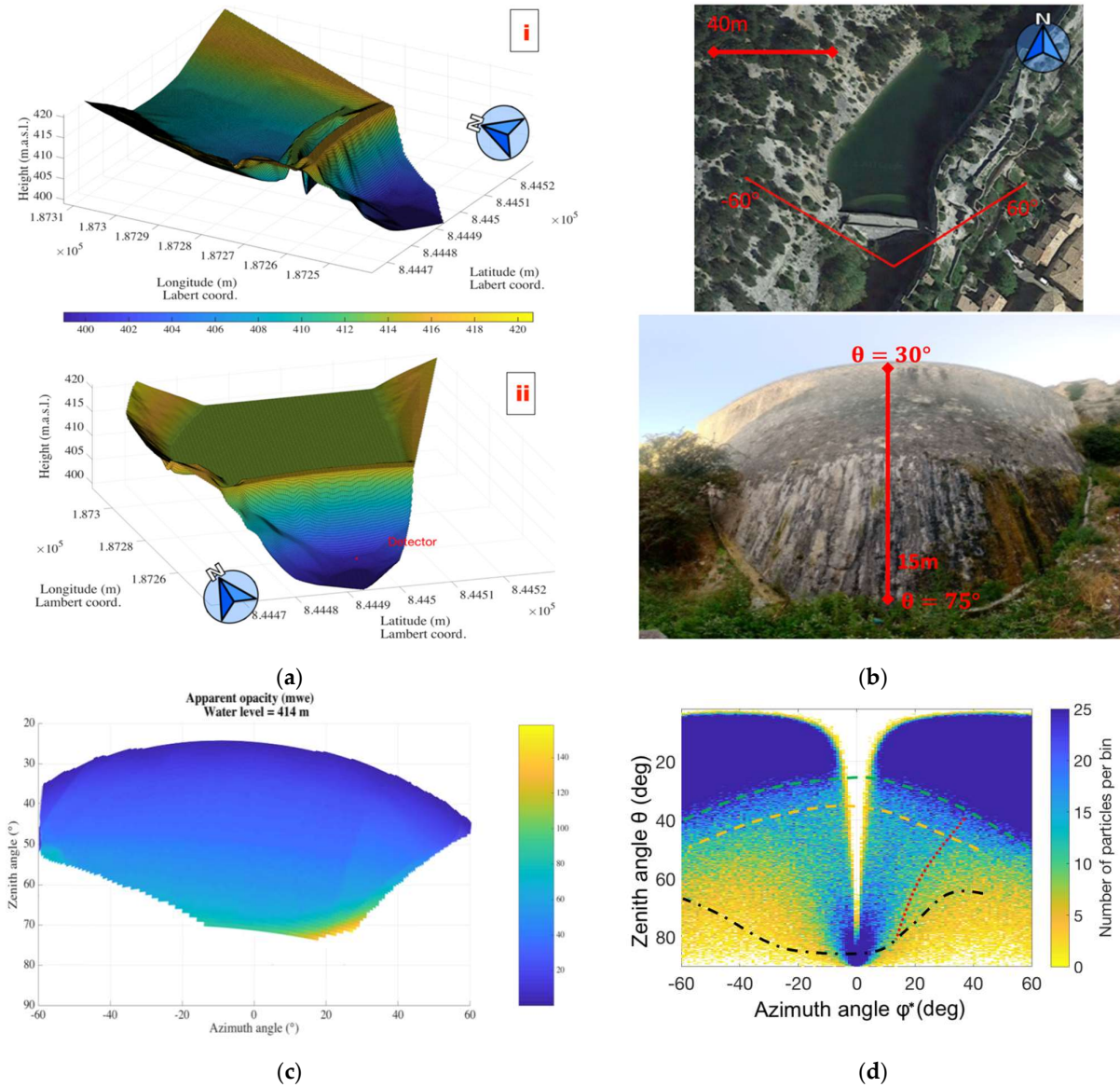
Figure 4. (a.i) Digital model of the empty water reservoir and (a.ii) filled with water at 414 m.a.s.l. (b) Approximation of the target volume as seen from the detector location. (c) Apparent opacity of the targeted volume with a water level of 414 m.a.s.l., the detector tilt was corrected. (d) Muons measured coming from the direction of the target volume.
