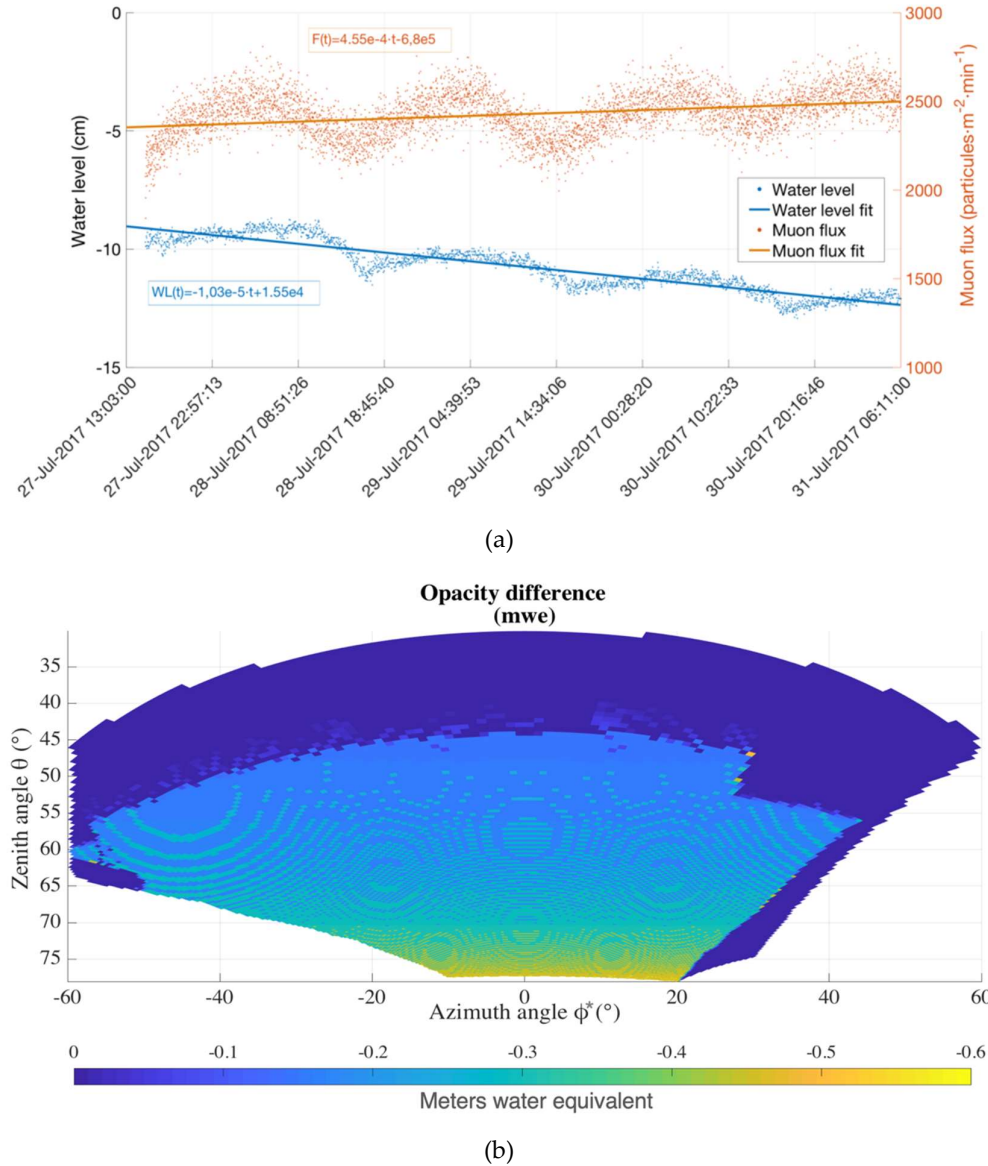
Figure 5. (a) Temporal evolution of (blue) water level of the dam and (orange) recorded muon flux and (b) change of apparent opacity of the medium due to the water transfer between the beginning and the end of the data acquisition.
