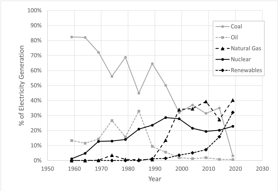
Figure 2. Graph showing mix of UK electricity over time. From the 1950s until 2000 coal was dominant (although in 2020 is now much less than 5%) In 2020, natural gas, wind/solar and nuclear were the main sources of electricity in the UK)
