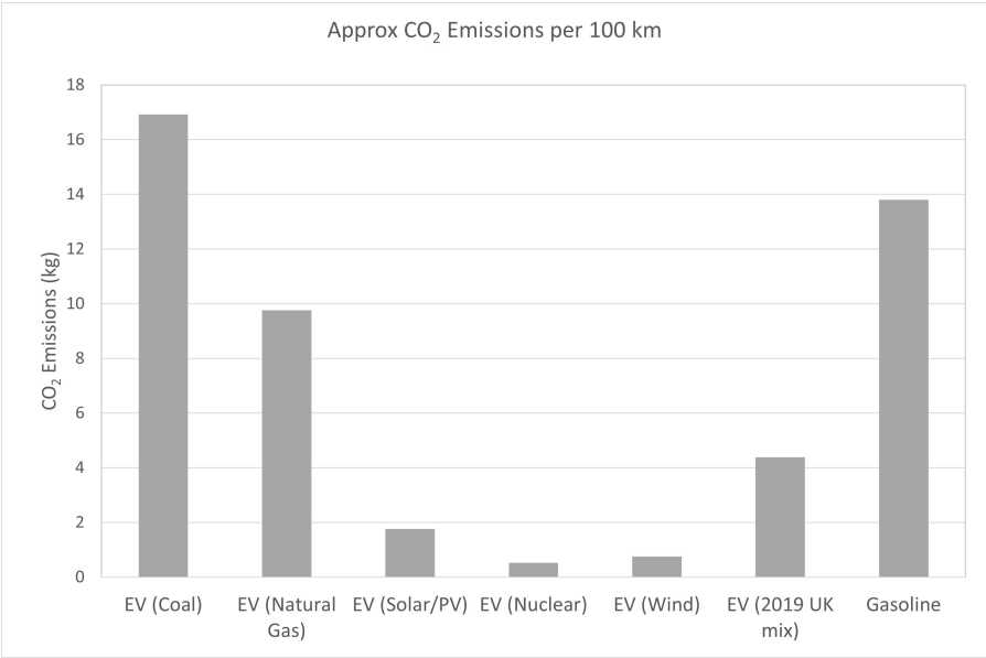
Figure 1. CO 2 emissions (in kg) for a car travelling 100 km. The electric vehicle emissions have assumed 20 kWh per 100 km, and for the gasoline car it was assumed the fuel consumption was 6 litres/100 km
