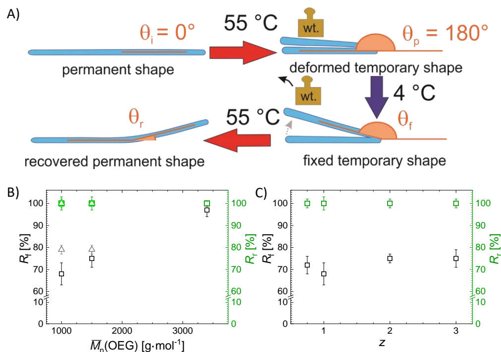
Figure 6. Shape-memory properties determined by bending experiments with temperature as stimulus. A) Schematic illustration of the experimental setup for the determination of shape fixity and shape recovery ratios. B) R_f and R_r as a function of OEG chain length for G20_OEGy(z) hydrogels ( \square : z = 1, \triangle : z = 2). C) R_f and R_r as a function of OEG content for G20_OEG1000(z) hydrogels.
