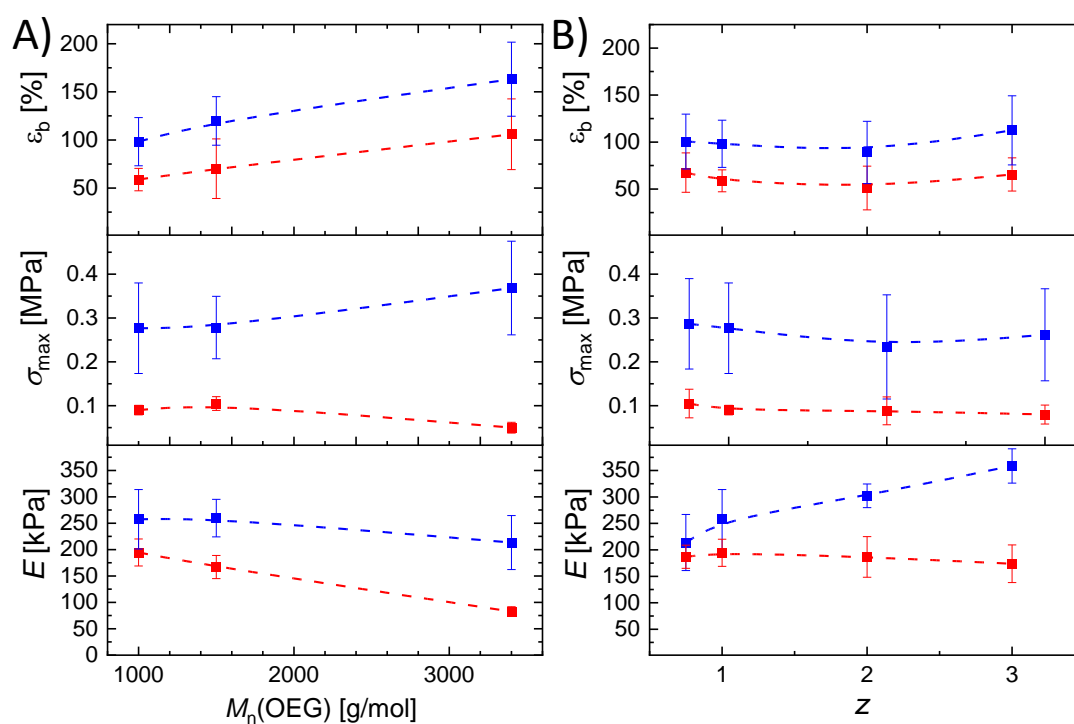
Figure 4. Elongation at break ( \varepsilon_b ), tensile strength ( \sigma_{max} ), and Young's modulus ( E ) of the gelatin based hydrogels under variation of OEG number average molar mass (A) or thiol:alkene molar ratio of the G20_OEG1000( z ) hydrogels (B), determined in tensile tests at 4 °C (blue) and 55 °C (red) in a water chamber. The lines are added as guide to the eye.
