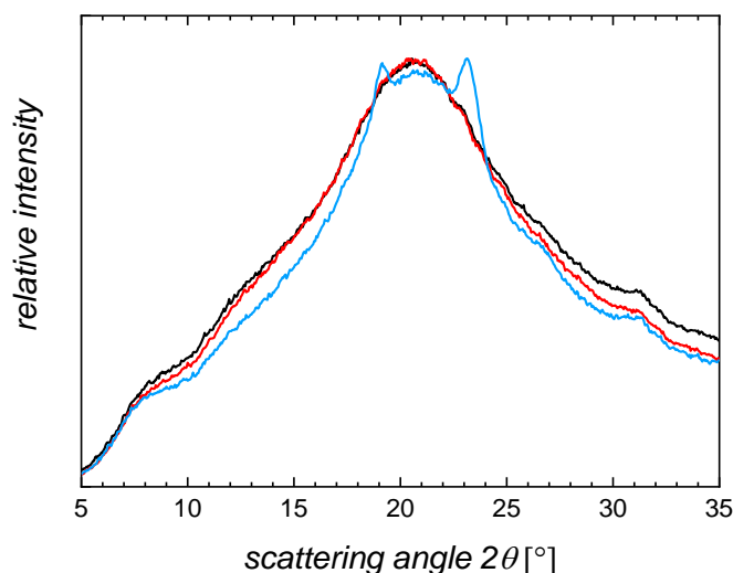
Figure 2. WAXS curves of dried G20_OEG1000(1) (black), G20_OEG1500(1) (red), and G20_OEG3400(1) (blue) networks at ambient temperature.
